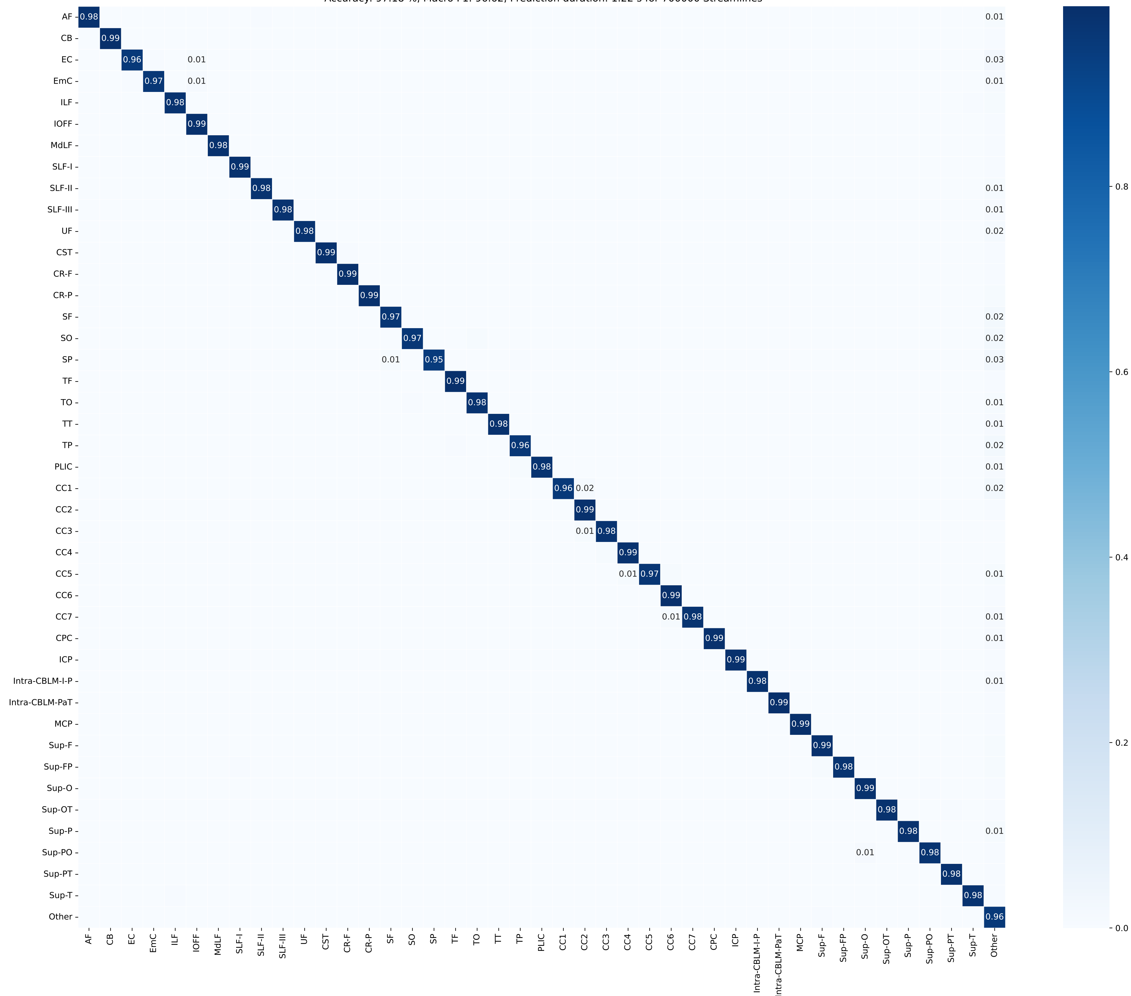
Confusion Matrix for all Subjects Accuracy: 97.18 %, Macro F1: 96.62, Prediction duration: 1.22 s for 700000 Streamlines
