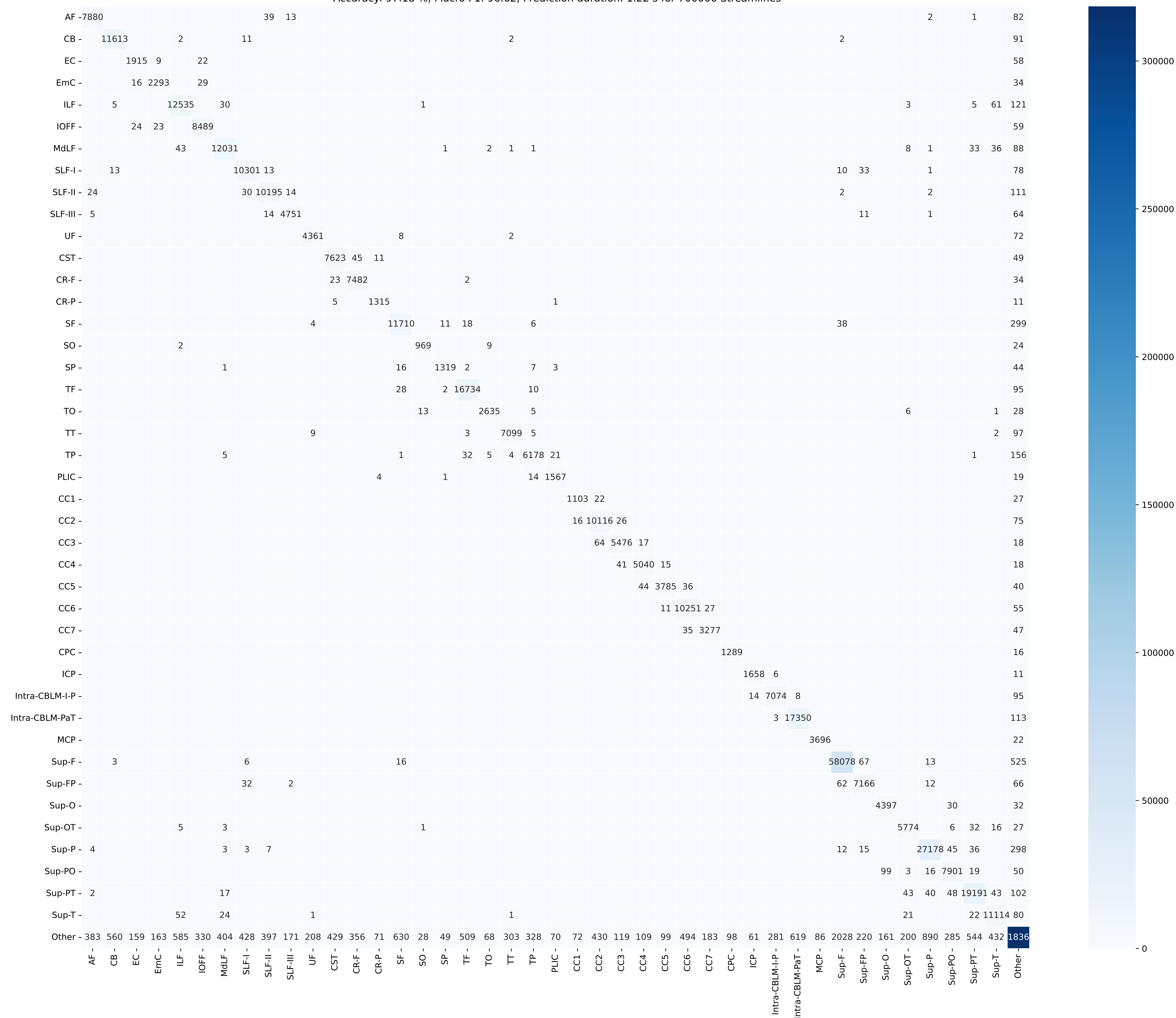
Unnormalized Confusion Matrix for all Subjects Accuracy: 97.18 %, Macro F1: 96.62, Prediction duration: 1.22 s for 700000 Streamlines
