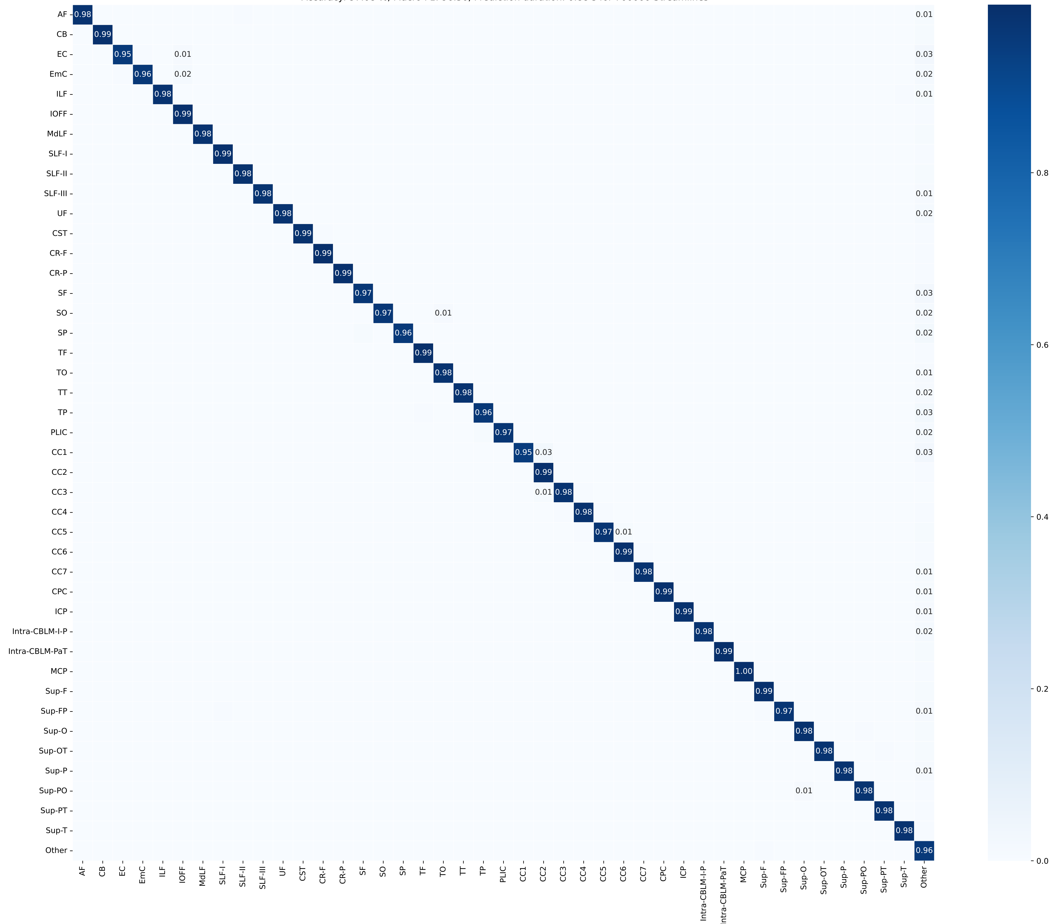
Confusion Matrix for all Subjects Accuracy: 97.08 %, Macro F1: 96.50, Prediction duration: 0.88 s for 700000 Streamlines
