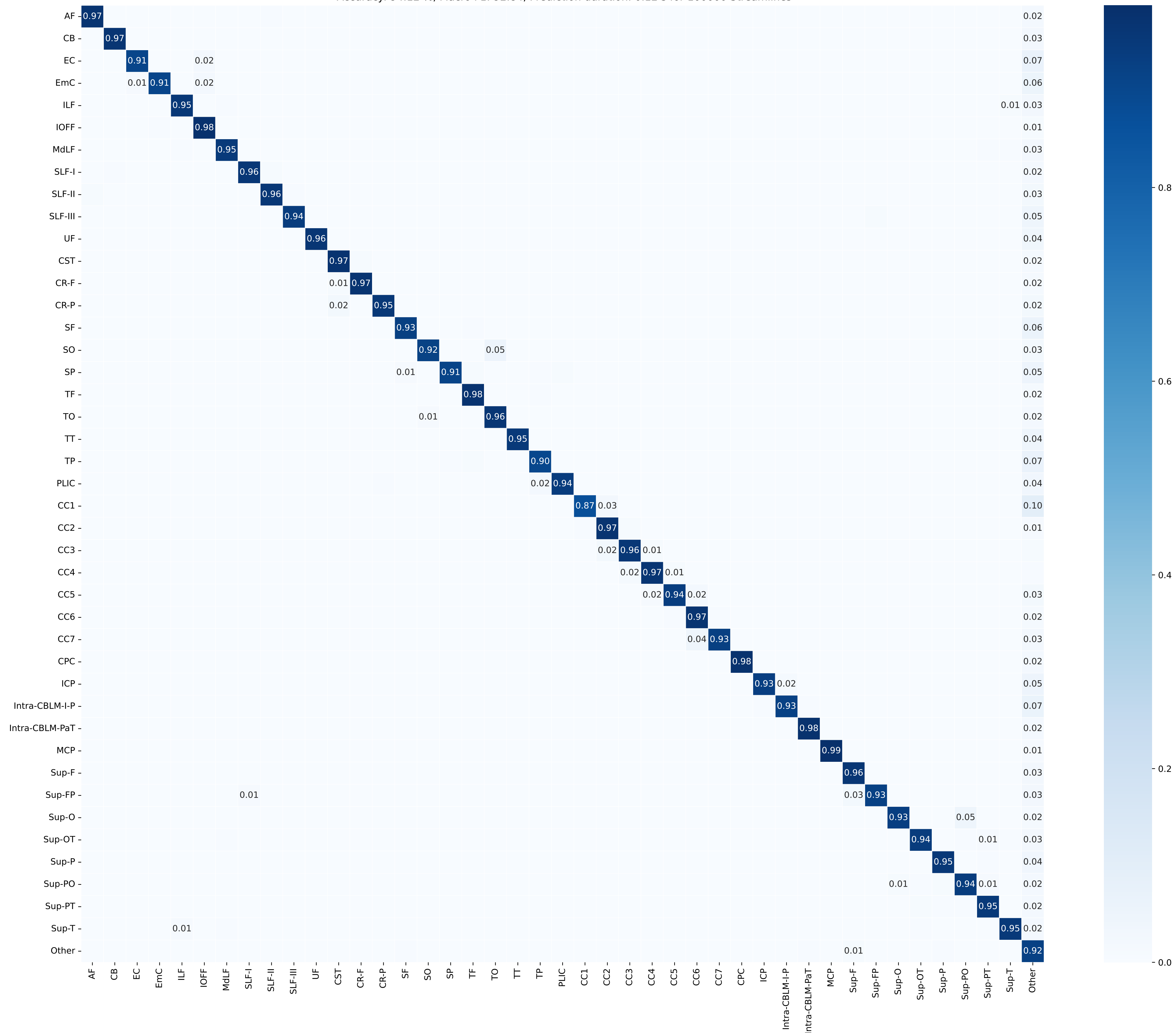
Confusion Matrix for all Subjects Accuracy: 94.12 %, Macro F1: 92.84, Prediction duration: 0.12 s for 100000 Streamlines
