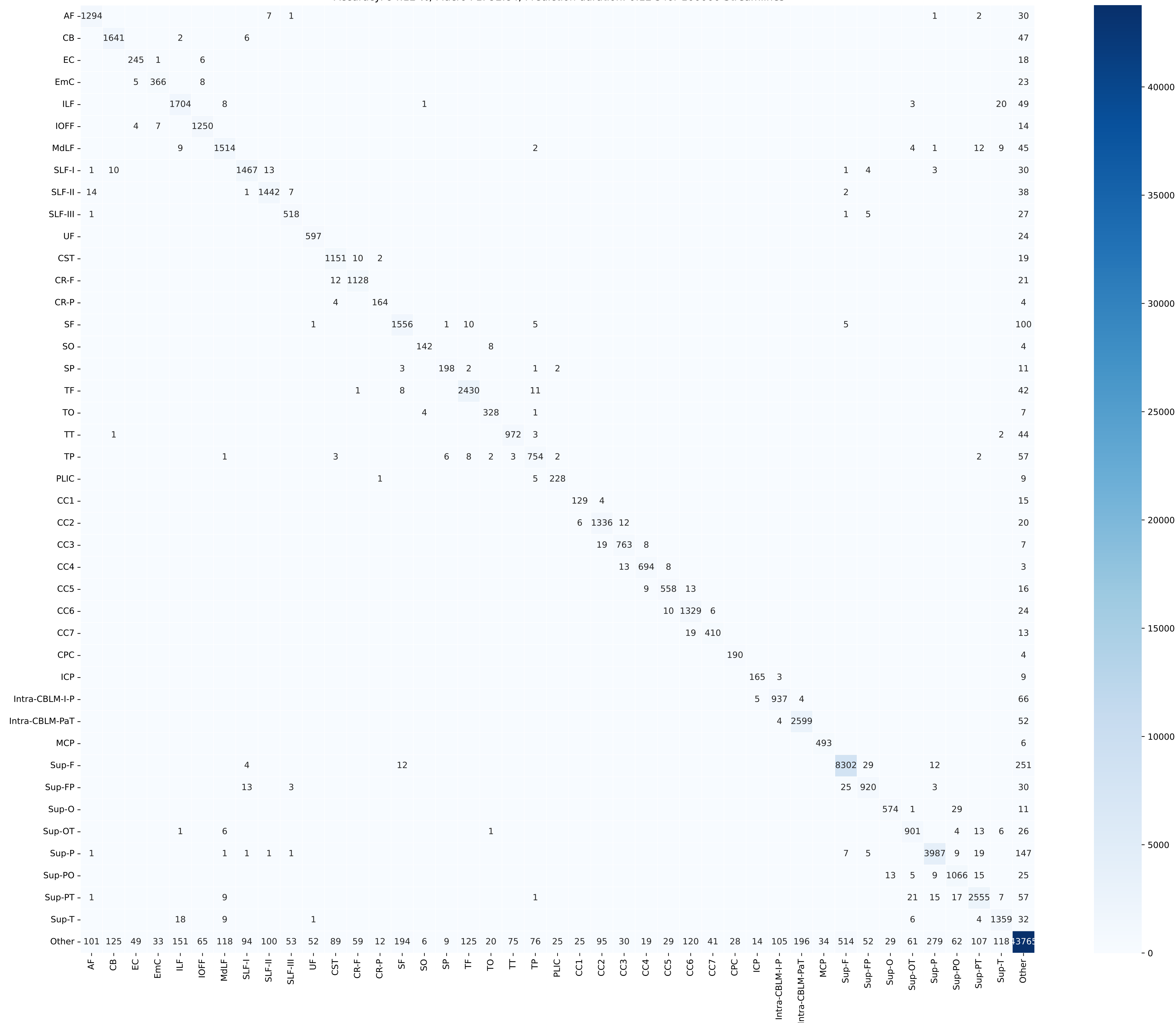
Unnormalized Confusion Matrix for all Subjects Accuracy: 94.12 %, Macro F1: 92.84, Prediction duration: 0.12 s for 100000 Streamlines
