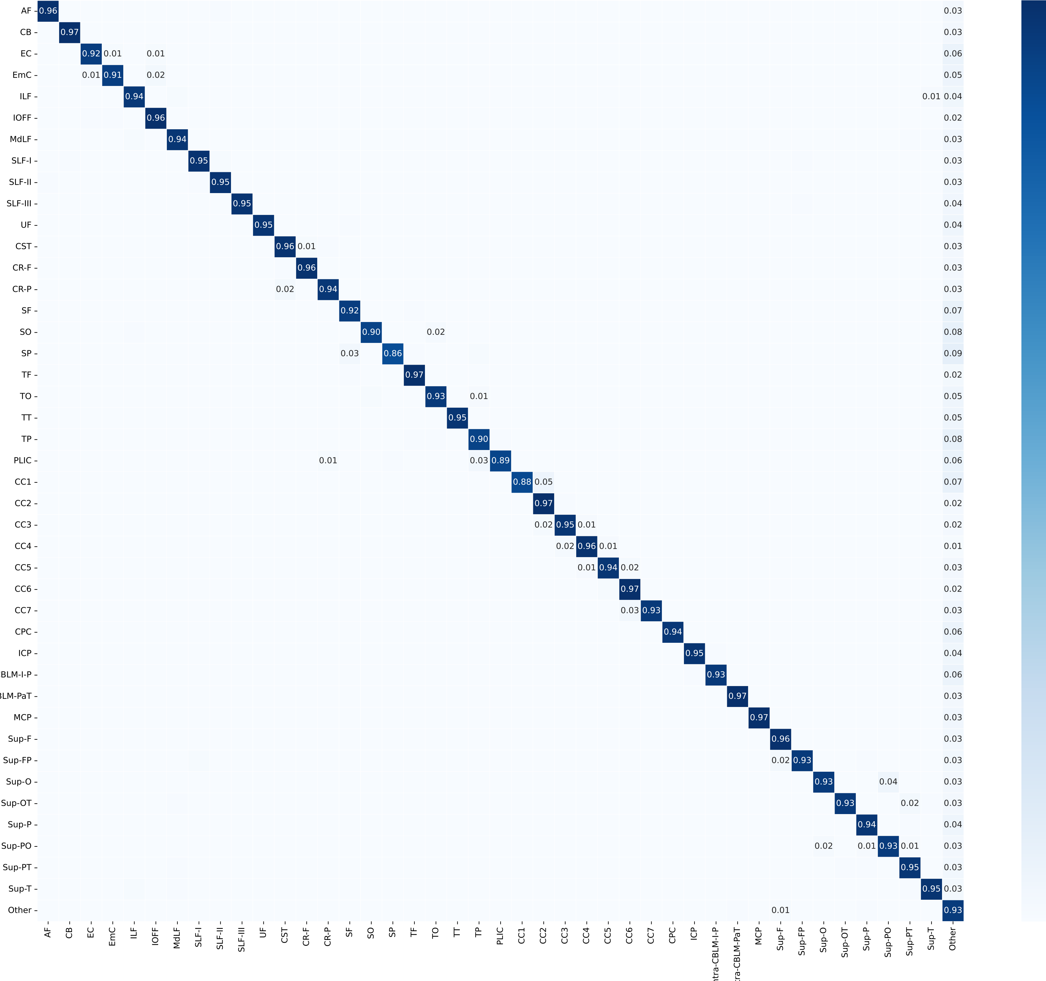
Confusion Matrix for all Subjects Accuracy: 93.81 %, Macro F1: 92.38, Prediction duration: 5.54 s for 6200000 Streamlines
