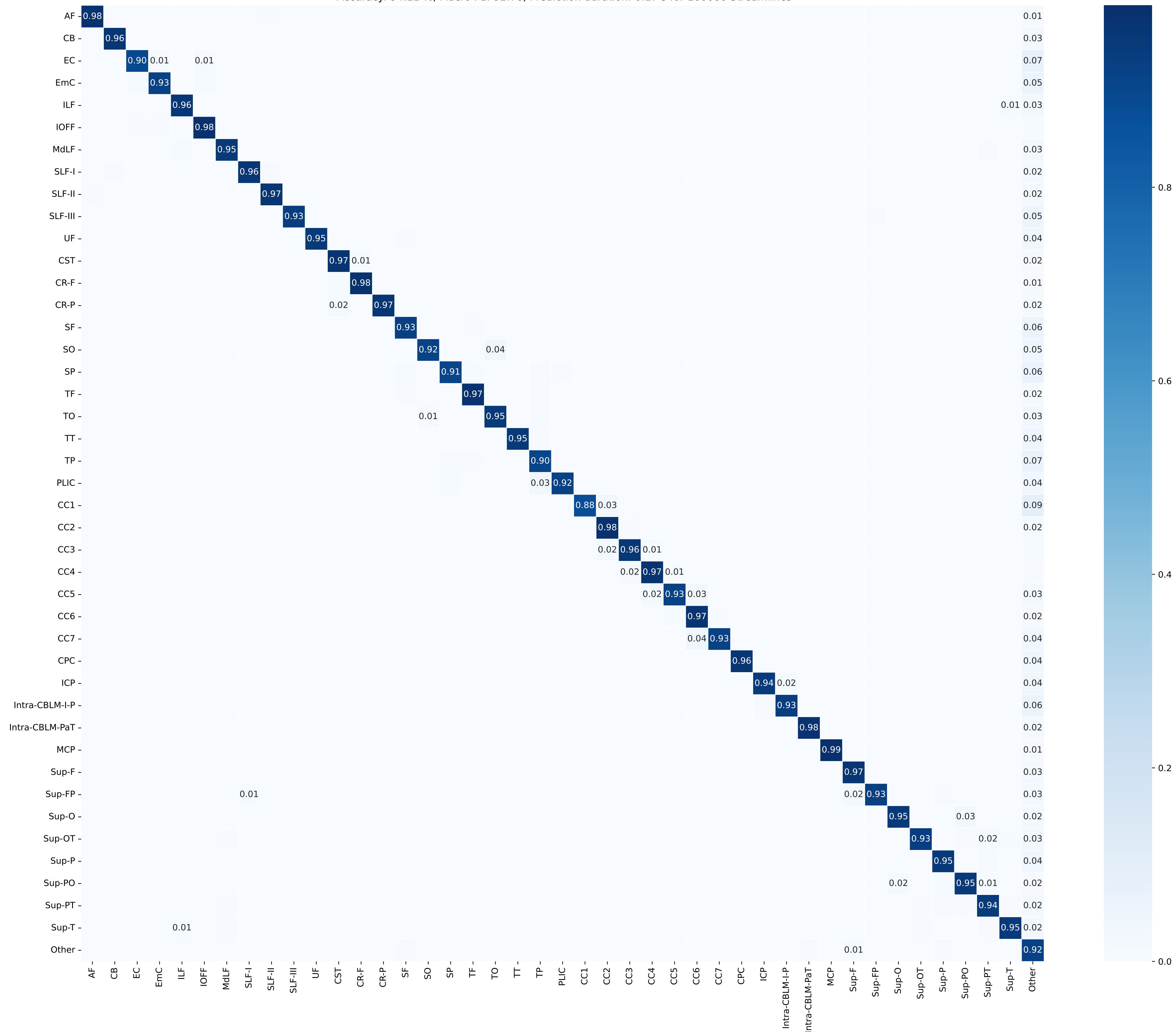
Confusion Matrix for all Subjects Accuracy: 94.11 %, Macro F1: 92.78, Prediction duration: 0.17 s for 100000 Streamlines
