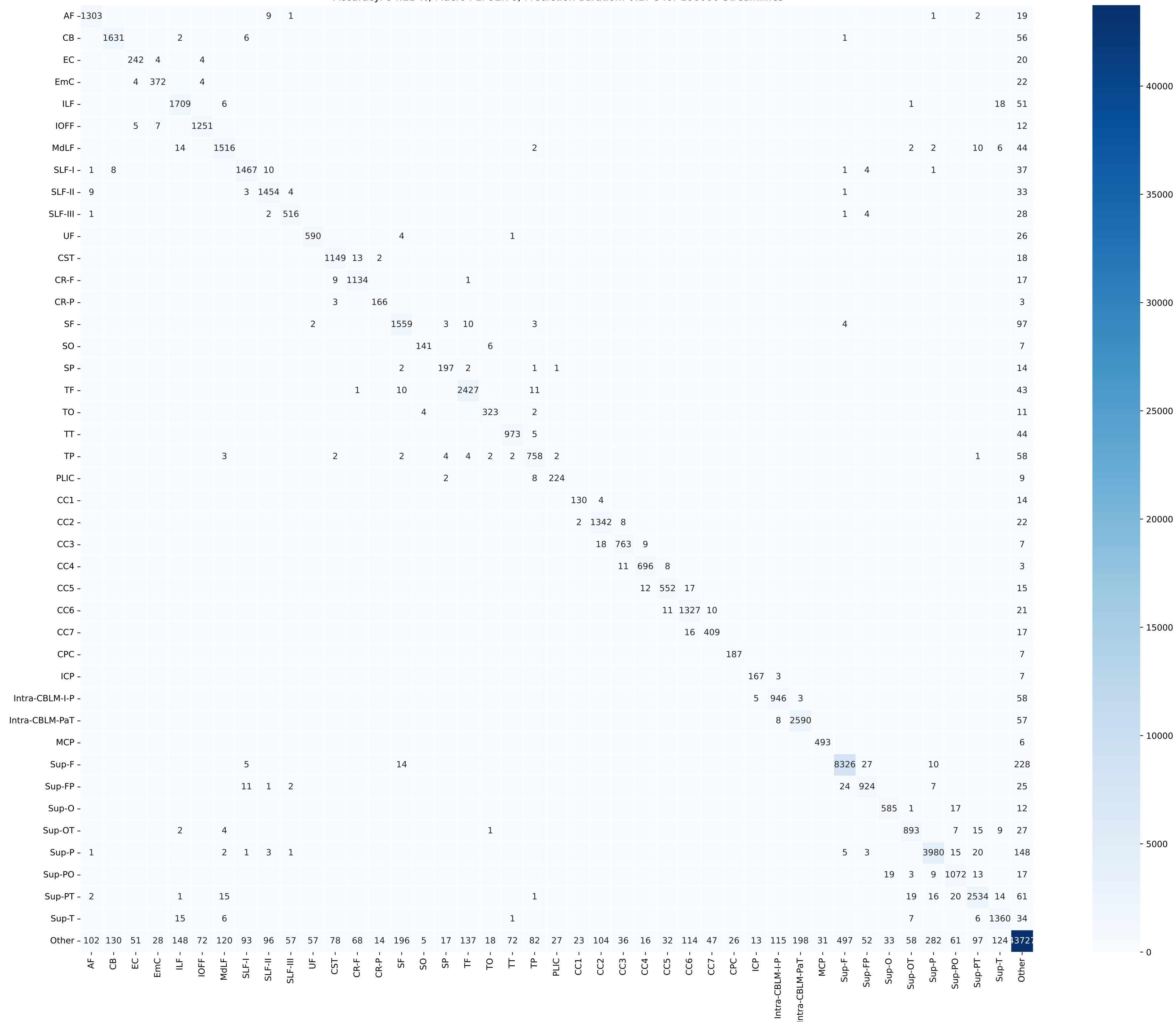
Unnormalized Confusion Matrix for all Subjects Accuracy: 94.11 %, Macro F1: 92.78, Prediction duration: 0.17 s for 100000 Streamlines
