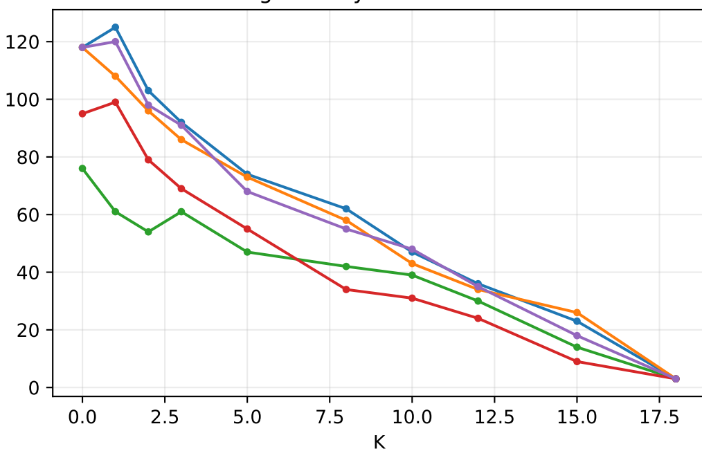
New geometry failures vs Exact
