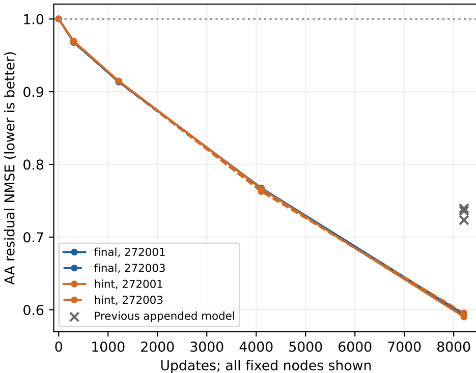
1W53 T37 TRAIN fit: same 8208-update budget, no transfer claim
