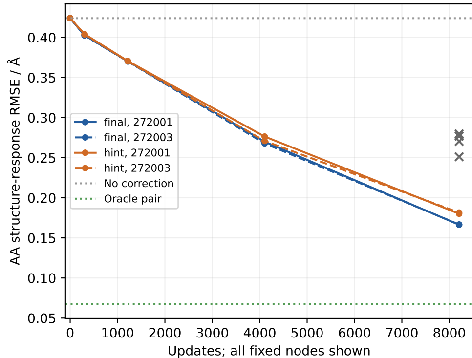
1W53 T37 TRAIN fit: same 8208-update budget, no transfer claim
