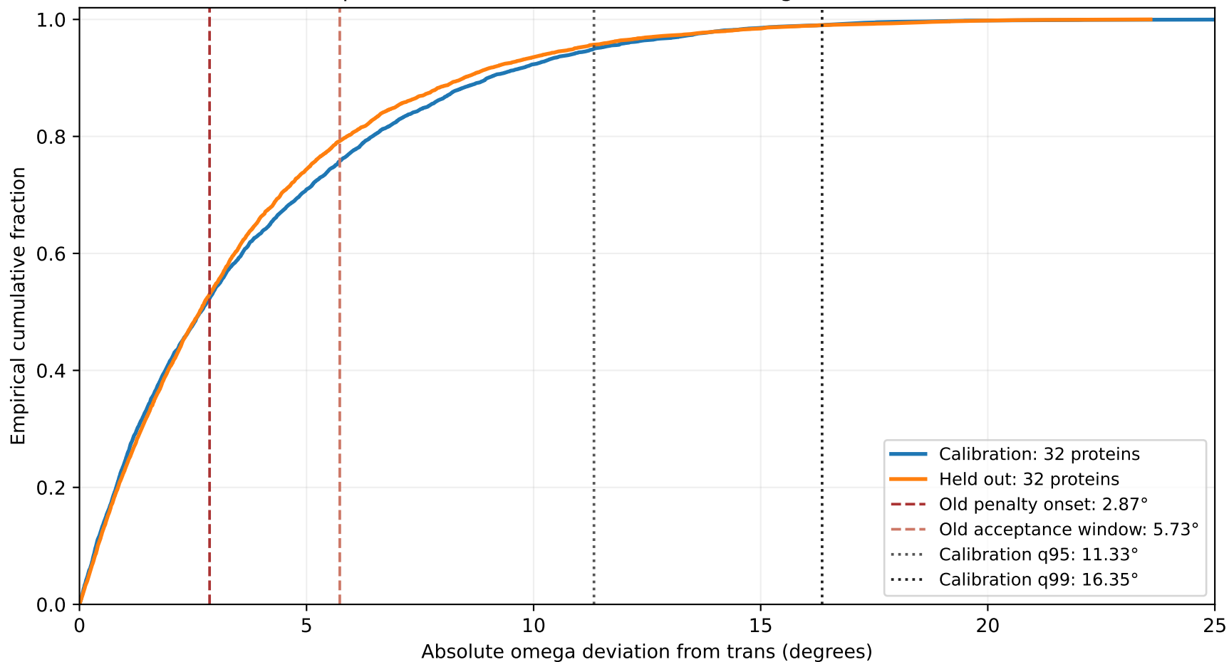
Experimental trans connections, following non-Pro residue
