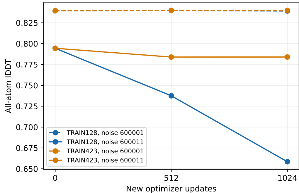
1MV8: post-hoc worst TRAIN128 change
