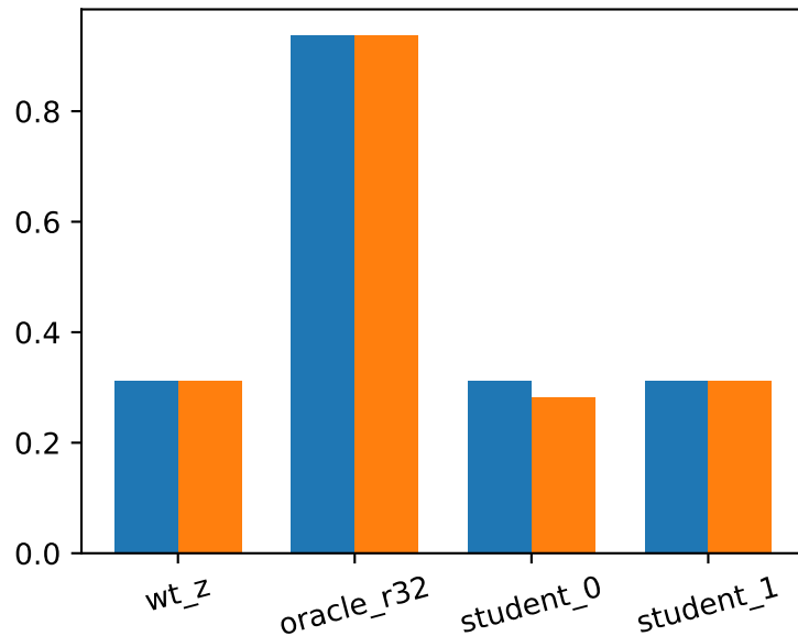
Top1 agreement
