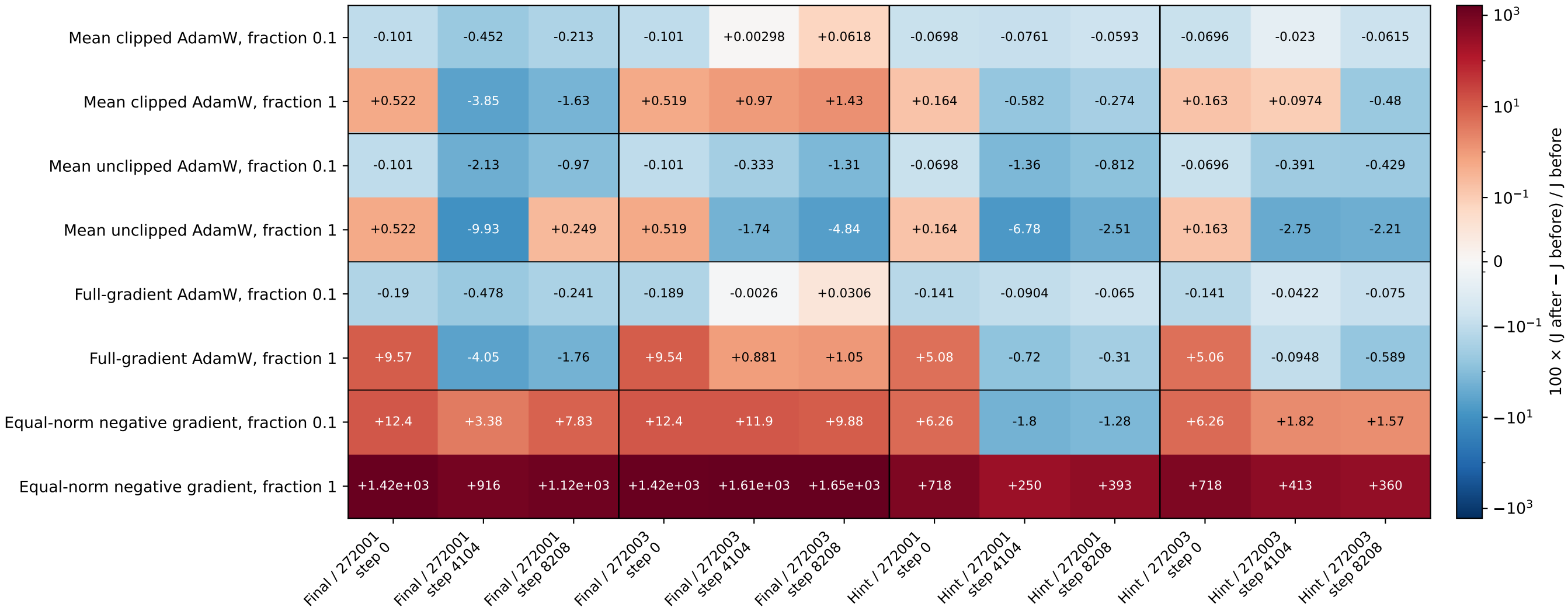
Full TRAIN objective change (%) at all fixed states Blue: lower loss; red: higher loss. Symmetric-log color scale; exact values annotated.
