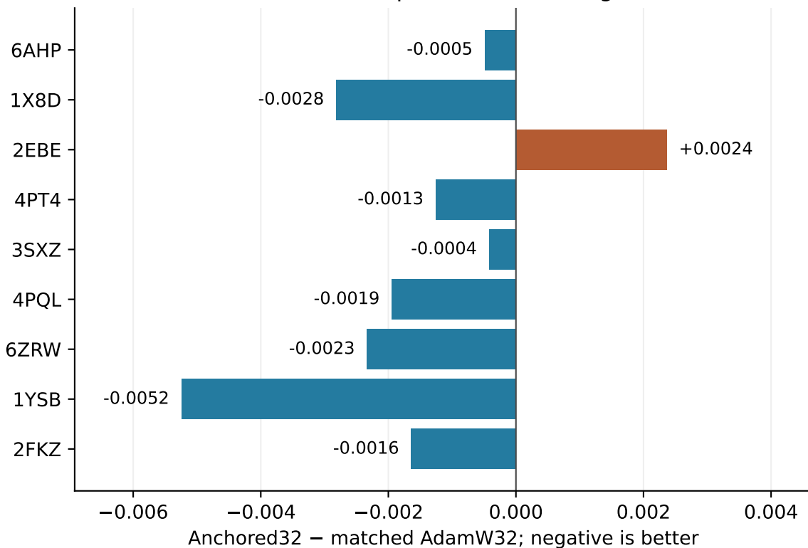
AA distance response RMSE change (Å)
