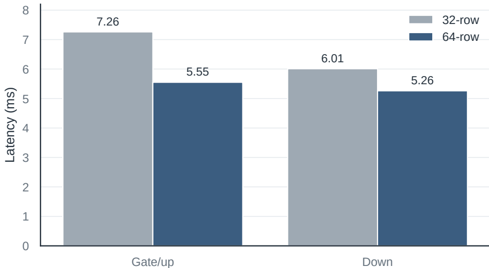
M2048 routed-MoE kernel latency
