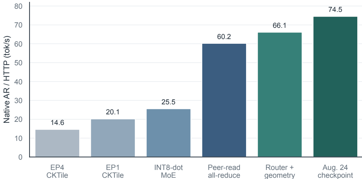
Historical TP4 single-request milestones (different checkpoints)
