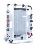
F1-22-MKII ENERGY LOSSES IN BENDS AND FITTINGS
