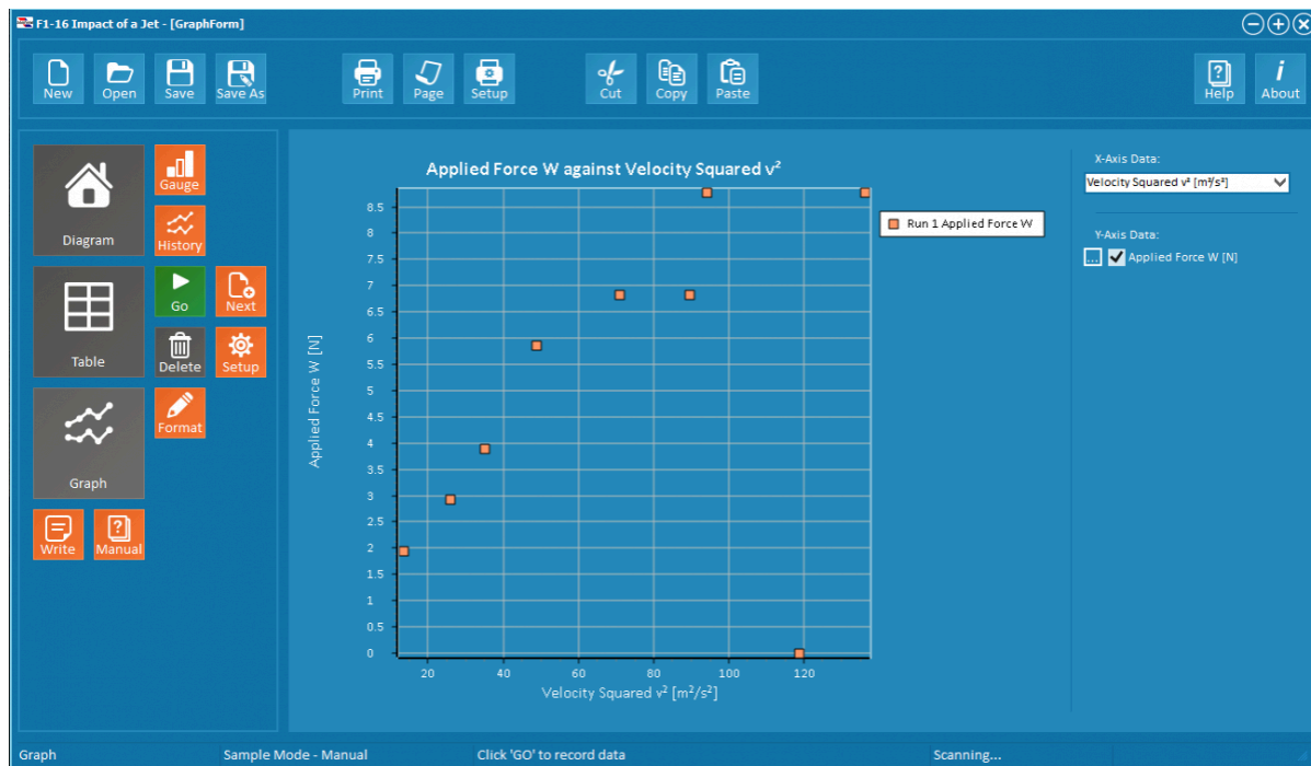
F1-16-MKII Impact of a Jet Graphical Display
