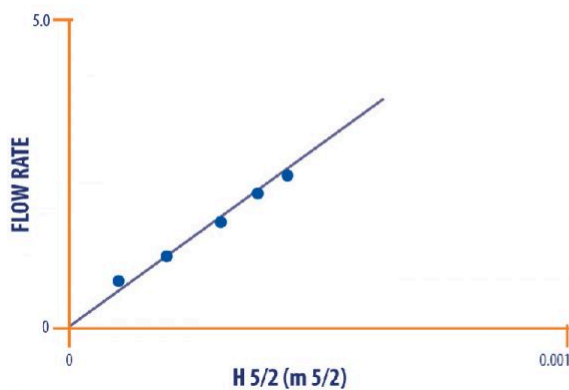
Armfield – F1-13-MKII Flow Over Weirs Graph
