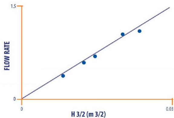
Armfield – F1-13-MKII Flow Over Weirs Graph
