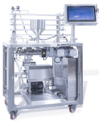
FT74XA HTST/UHT SYSTEM
