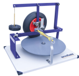
SD-1.57 – CASTOR, CAMBER AND KING PIN INCLINATION
