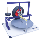
SD-1.57 – CASTOR, CAMBER AND KING PIN INCLINATION
