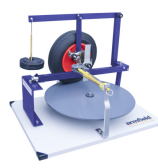
SD-1.57 – CASTOR, CAMBER AND KING PIN INCLINATION
