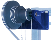
SD-1.51 – WHEEL AND DIFFERENTIAL AXLE APPARATUS
