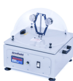
SD-1.61 – GOVERNOR APPARATUS
