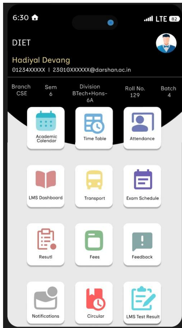
Home Screen
