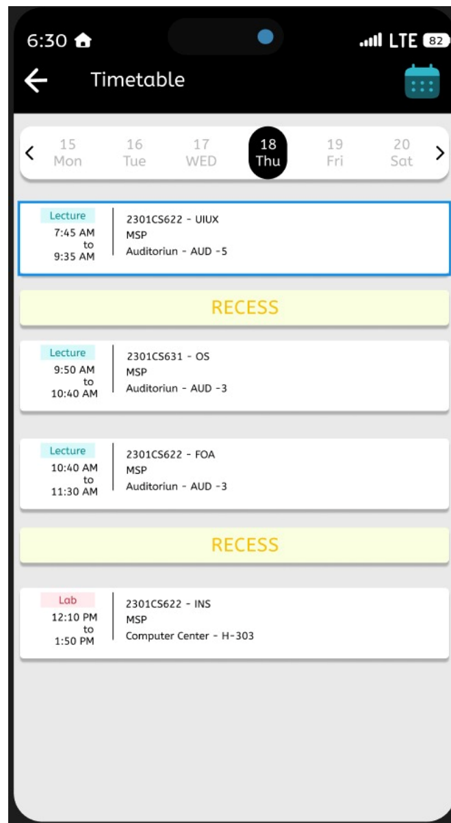
Time-Table Screen
