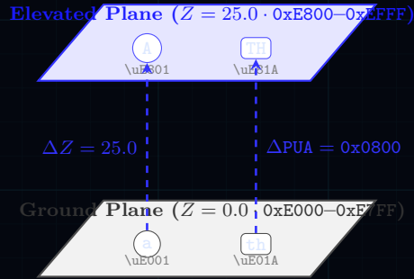
Figure 3: Dual-Plane Semiotic Casing Architecture. Base lowercase glyphs and compound chords populate the Ground Plane ( Z = 0.0 ), while uppercase and emphatic tokens occupy the Elevated Plane ( Z = 25.0 ) via an exact isometric translation.
