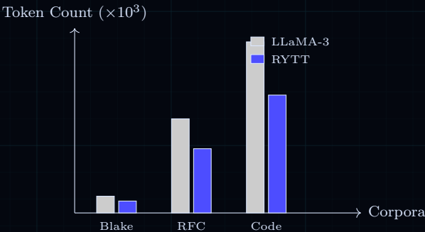
Figure 4: Compression efficiency comparison: RYTT was previously claimed to achieve a 24.8%–31.2% reduction in sequence length over modern subword tokenizers; independent measurement against tiktoken instead found 4–11× MORE tokens. [retracted].
