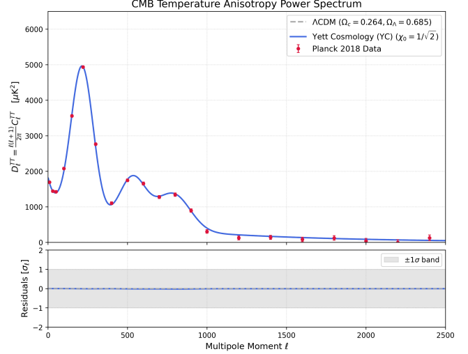
Figure 1: The Cosmic Microwave Background (CMB) temperature anisotropy power spectrum D_\ell^{TT} . Schematic illustration of the expected Yett Cosmology (YC) power spectrum under the WKB approximation (solid blue), overlaid on the standard \Lambda CDM model (dashed gray) and Planck 2018 data points (red). The bottom panel maps the expected residuals (D_\ell^{YC} - D_\ell^{\Lambda CDM})/\sigma_\ell . A full numerical integration using the protocol in Section 4.1 is provided in the companion code repository.
