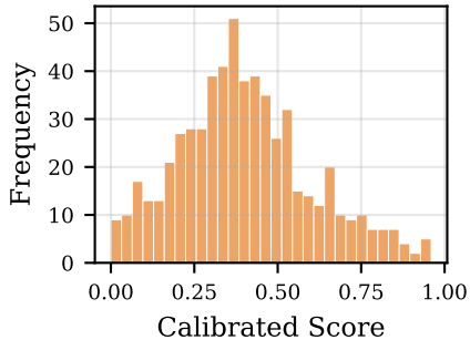
Negative Arousal
