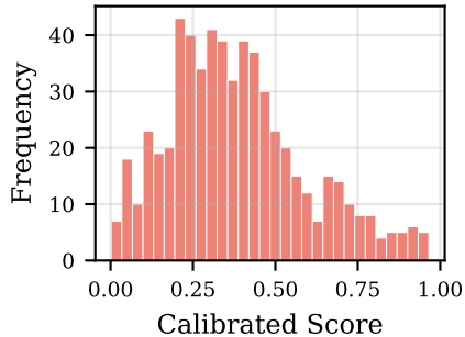
Attack Intensity
