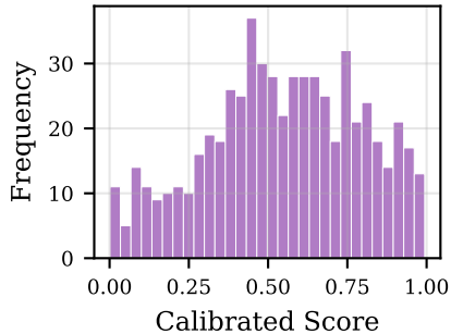
Stance Polarization
