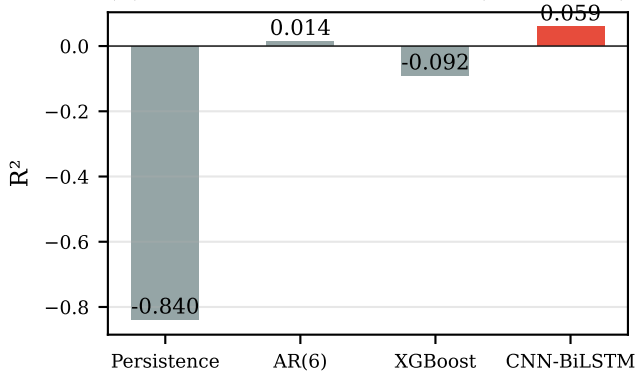
(a) Conflict-Index Forecast (Real Data)
