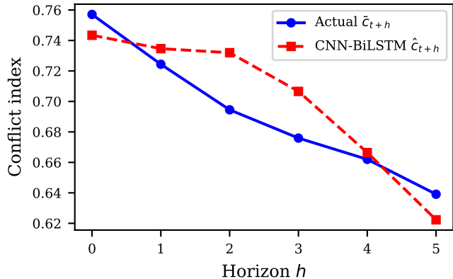
(b) Multi-step forecast sample
