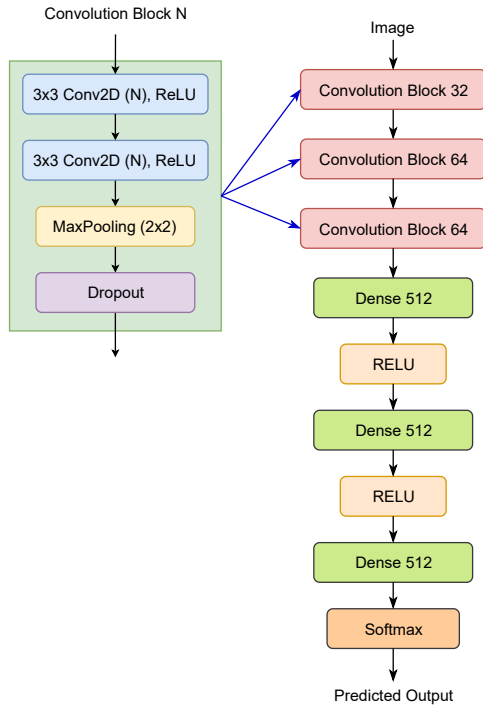
Figure 7: Details of the CNN layers
