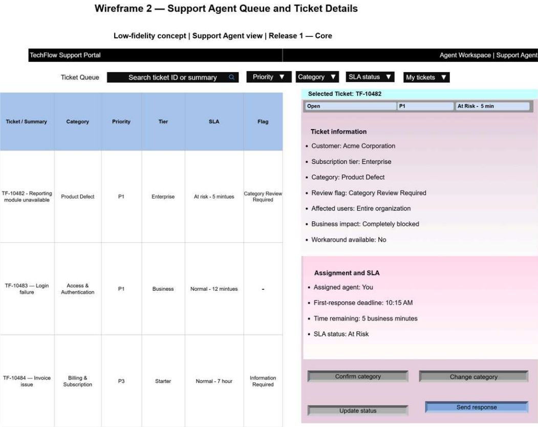
Figure 2. Low-fidelity Support Agent queue and ticket details concept
