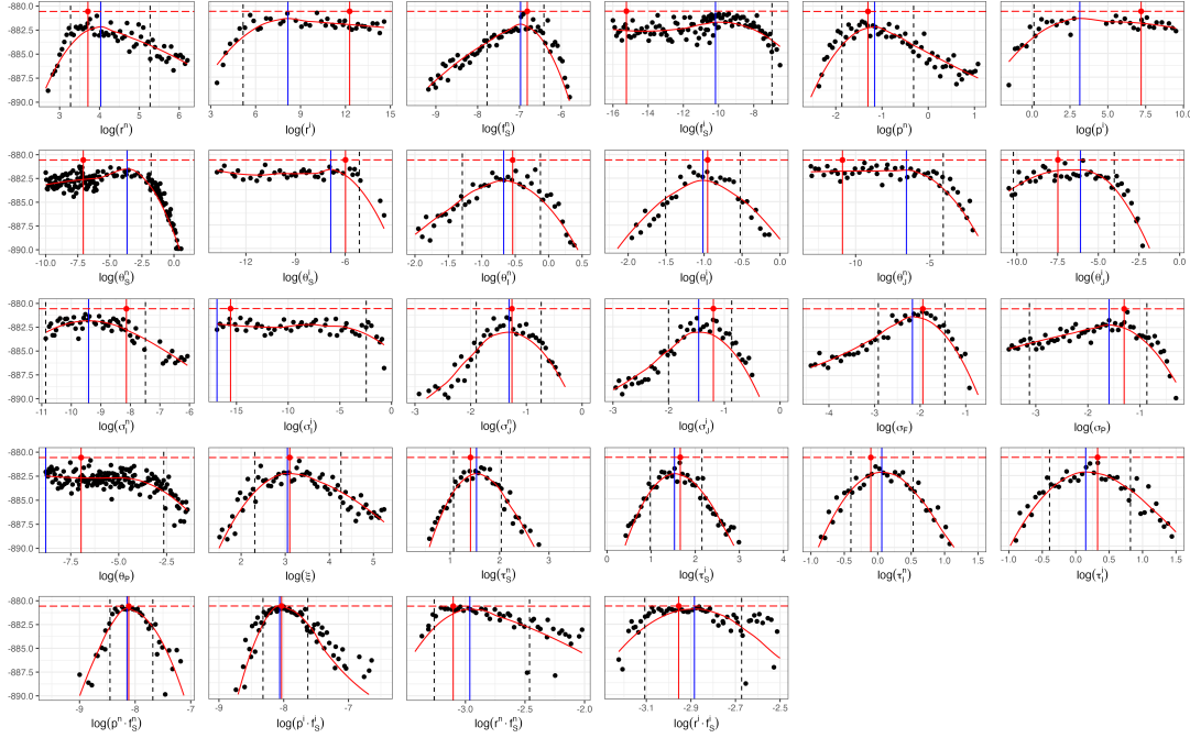
Figure S-2: Monte Carlo Adjusted Profile results of SIRJPF2 model for mixed species Parasitized dynamics. The vertical dotted lines represent the 95% confidence interval obtained by MCAP. The vertical blue lines show the MLE estimated using MCAP. The red vertical lines correspond to the model with the overall highest likelihood among all searches.
