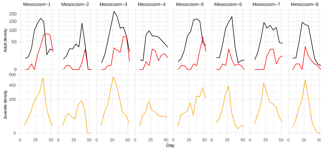
Figure S-6: Density (Individuals/Liter) of D. dentifera . The top panel shows adult susceptibles ( D. dentifera , black) and infecteds ( D. dentifera , red). The bottom panel shows juvenile susceptibles ( D. dentifera , orange). There were negligible infected juveniles. Columns are buckets corresponding to replications with same treatment setting.
