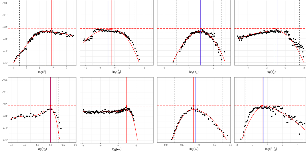
Figure S-23: Monte Carlo Adjusted Profile results of SRJF model for D. lumholtzi -only dynamics. The vertical dotted lines represent the 95% confidence interval obtained by MCAP. The vertical blue lines show the MLE estimated using MCAP. The red vertical lines correspond to the model with the overall highest likelihood among all searches.
