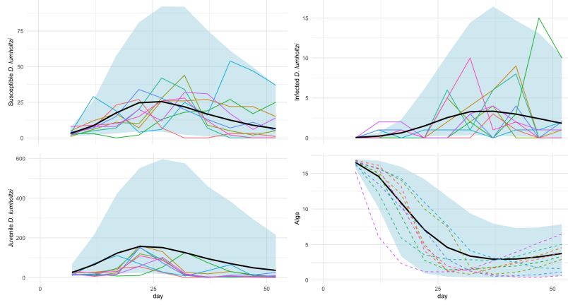
Figure S-12: Simulation plots of densities (Individuals/Liter) for susceptible, infected, and juvenile D. lumholtzi , along with alga density ( 10^6 \cdot \text{cells/Liter} ) and parasite density ( 10^3 \cdot \text{spores/Liter} ), over time (days). The colorful solid lines represent observed experimental data, showing the variability across different experimental replicates. The black line represents the mean trajectory from the simulation model, capturing the general trend of each density. The light blue shaded area corresponds to the 95% confidence interval of the simulations, indicating the range of model predictions. Dashed lines illustrate individual simulated trajectories, highlighting the model's ability to capture fluctuations around the mean trajectory.
