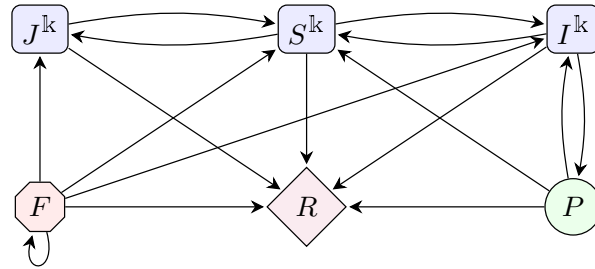
Figure S-5: Flow diagram for the SIRJPF model illustrating population interactions. The model includes the R state, representing mortality. Susceptible populations ( S^k ) can reproduce into juvenile ( J^k ), where the superscript k denotes the species of Daphnia . And A. Algae ( F ) will be refilled, as shown by the recycling arrows. Transitions from S^k to I^k denote infection, and transitions to the R state occur upon death, where deceased individuals release parasites back into the environment. All S^k , I^k and J^k consume resources from F , and over time, components in F and P also progress to R .
