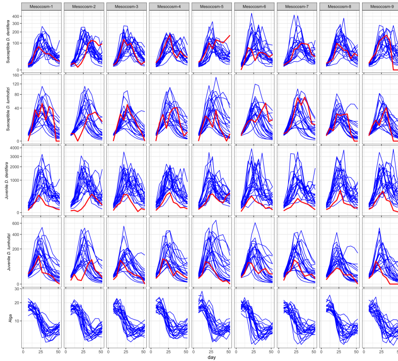
Figure S-18: Simulated density ( 10^6 cells/Liter) of susceptible native D. dentifera , susceptible invasive D. lumholtzi , juvenile native D. dentifera , invasive D. lumholtzi , and alga density ( F ) over time (days) for each experimental unit. The blue lines represent individual simulation cases, while the red line denotes observed experimental data, showing how simulated variability compares to actual data.
