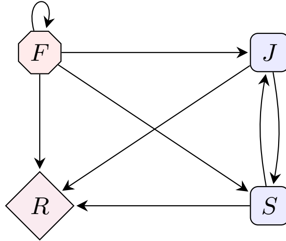
Figure S-19: Flow diagram for the SRJF model illustrating population interactions. The model includes the R state, representing mortality. For \mathbb{k} \in \{\mathfrak{n}, \mathfrak{i}\} , susceptible populations ( S^{\mathbb{k}} ) can reproduce into juvenile ( J^{\mathbb{k}} ) and A . Algae ( F ) will be refilled, as shown by the recycling arrows. Both S^{\mathbb{k}} and J^{\mathbb{k}} consume resources from F , and over time, components in F also progress to R .
