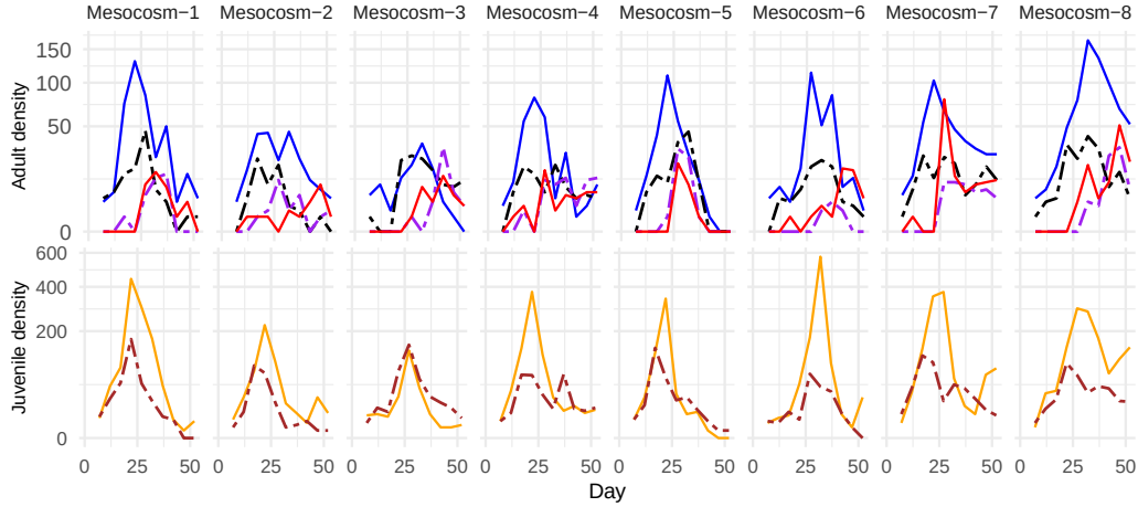
Figure 1: The experimental data. Density (Individuals/Liter) of D. dentifera (solid lines) and D. lumholtzi (dashed lines). The top panel shows adult susceptibles ( D. dentifera , blue; D. lumholtzi , black) and infecteds ( D. dentifera , red; D. lumholtzi , purple). The bottom panel shows juvenile susceptibles ( D. dentifera , orange; D. lumholtzi , brown). There were negligible infected juveniles. Columns are buckets corresponding to replications with same treatment setting.
