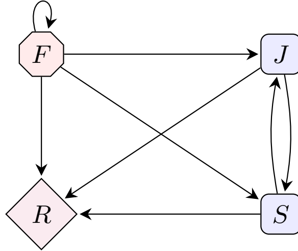
Figure S-18: Flow diagram for the SRJF model illustrating population interactions. The model includes the R state, representing mortality. For \mathbb{k} \in \{\mathbb{m}, \mathbb{i}\} , susceptible populations ( S^{\mathbb{k}} ) can reproduce into juvenile ( J^{\mathbb{k}} ) and A. Algae ( F ) will be refilled, as shown by the recycling arrows. Both S^{\mathbb{k}} and J^{\mathbb{k}} consume resources from F , and over time, components in F also progress to R .
