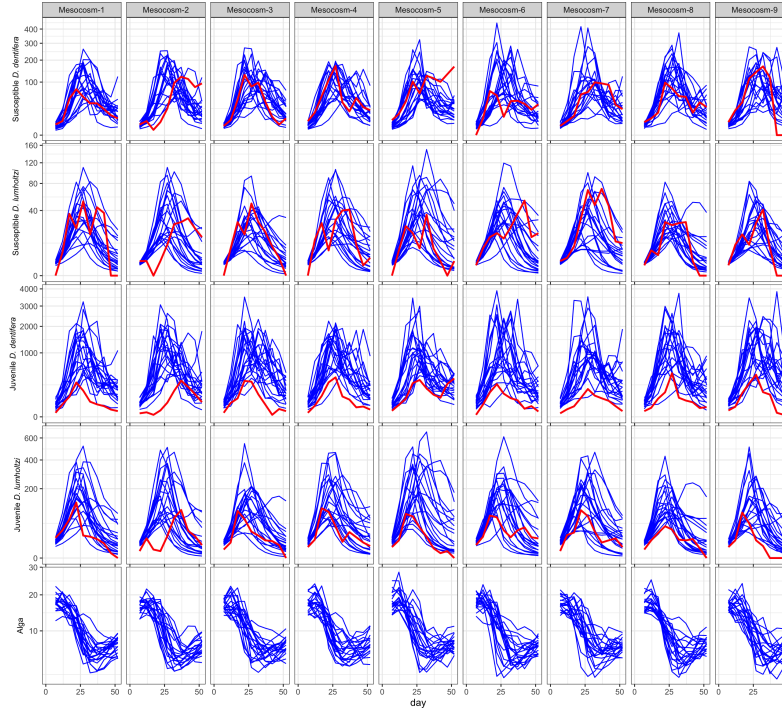
Figure S-17: Simulated density ( 10^6 cells/Liter) of susceptible native D. dentifera , susceptible invasive D. lumholtzi , juvenile native D. dentifera , invasive D. lumholtzi , and algae density ( F ) over time (days) for each experimental unit. The blue lines represent individual simulation cases, while the red line denotes observed experimental data, showing how simulated variability compares to actual data.
