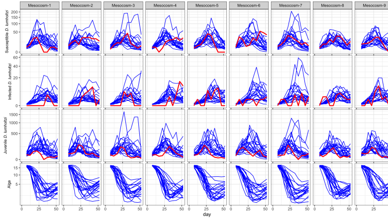
Figure S-12: Simulated trajectories of susceptible D. lumholtzi , infected D. lumholtzi , juvenile D. lumholtzi and alga density ( 10^6 \cdot \text{cells/Liter} ) over time (days) for each experimental unit (u1 to u9). The blue lines represent individual simulation runs, capturing the variability in susceptible density across replicates, while the red line represents the actual experimental data.
