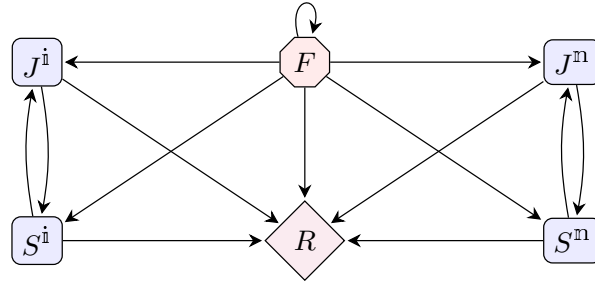
Figure S-13: Flow diagram for the SRJF2 model illustrating population interactions. The model includes the R state, representing mortality. For \mathbb{k} \in \{\mathfrak{m}, \mathfrak{i}\} , Susceptible populations ( S^{\mathbb{k}} ) can reproduce into juvenile ( J^{\mathbb{k}} ). And A. Algae ( F ) will be refilled, as shown by the recycling arrows. Both S^{\mathbb{k}} and J^{\mathbb{k}} consume resources from F , and over time, components in F also progress to R .
