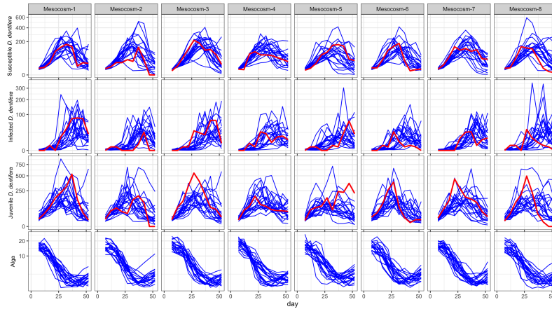
Figure S-10: Simulated densities (Individuals/Liter) of susceptible D. dentifera , infected D. dentifera density, juvenile D. dentifera and alga density ( 10^6 ·cells/Liter) over time (days) for each experimental unit. The blue lines represent individual simulation runs, capturing the variability in susceptible density across replicates, while the red line represents the actual experimental data.
