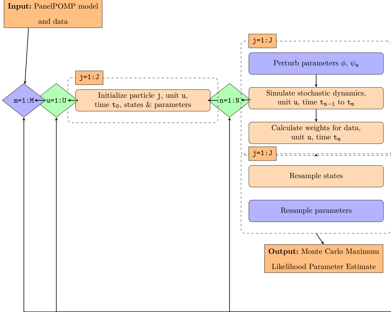
Figure 3: A flow diagram for panel iterated filtering. If the blue shaded blocks are omitted, this becomes a standard particle filter for each unit. Full pseudocode is in Section S2. In the PIF algorithm of Bretó et al. (2020) , the parameter resampling step involves re-selecting the unit-specific parameters corresponding to particle j for units \tilde{u} \neq u as well as \psi_u . For the marginalized PIF algorithm, only \phi and \psi_u are reselected in this step.
