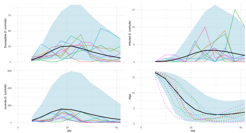
Figure S-11: Simulation plots of densities (Individuals/Liter) for susceptible, infected, and juvenile D. lumholtzi , along with alga density ( 10^6 ·cells/Liter) and parasite density ( 10^3 ·spores/Liter), over time (days). The colorful solid lines represent observed experimental data, showing the variability across different experimental replicates. The black line represents the mean trajectory from the simulation model, capturing the general trend of each density. The light blue shaded area corresponds to the 95% confidence interval of the simulations, indicating the range of model predictions. Dashed lines illustrate individual simulated trajectories, highlighting the model's ability to capture fluctuations around the mean trajectory.
