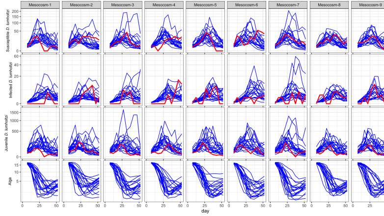
Figure S-12: Simulated trajectories of susceptible D. lumholtzi , infected D. lumholtzi , juvenile D. lumholtzi and alga density ( 10^6 ·cells/Liter) over time (days) for each experimental unit (u1 to u9). The blue lines represent individual simulation runs, capturing the variability in susceptible density across replicates, while the red line represents the actual experimental data.
