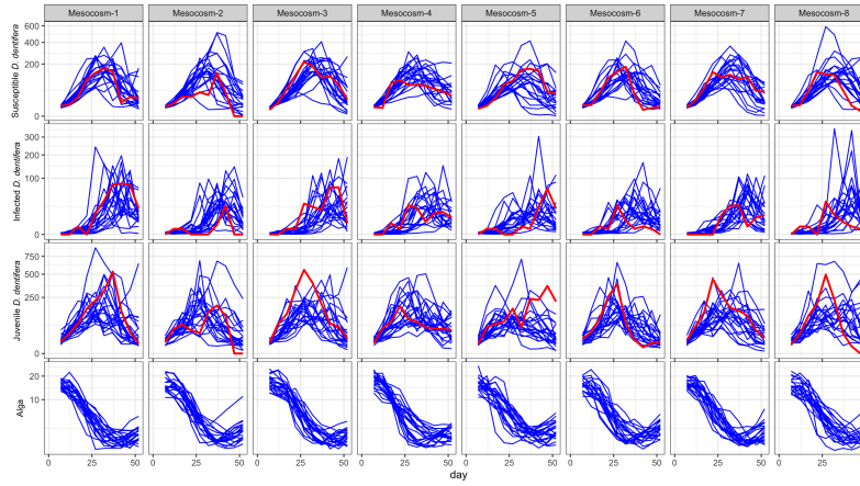
Figure S-10: Simulated densities (Individuals/Liter) of susceptible D. dentifera , infected D. dentifera density, juvenile D. dentifera and alga density ( 10^6 ·cells/Liter) over time (days) for each experimental unit. The blue lines represent individual simulation runs, capturing the variability in susceptible density across replicates, while the red line represents the actual experimental data.
