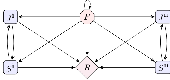
Figure S-13: Flow diagram for the SRJF2 model illustrating population interactions. The model includes the R state, representing mortality. For \mathfrak{k} \in \{\mathfrak{n}, \mathfrak{i}\} , Susceptible populations ( S^{\mathfrak{k}} ) can reproduce into juvenile ( J^{\mathfrak{k}} ). And A. Algae ( F ) will be refilled, as shown by the recycling arrows. Both S^{\mathfrak{k}} and J^{\mathfrak{k}} consume resources from F , and over time, components in F also progress to R .
