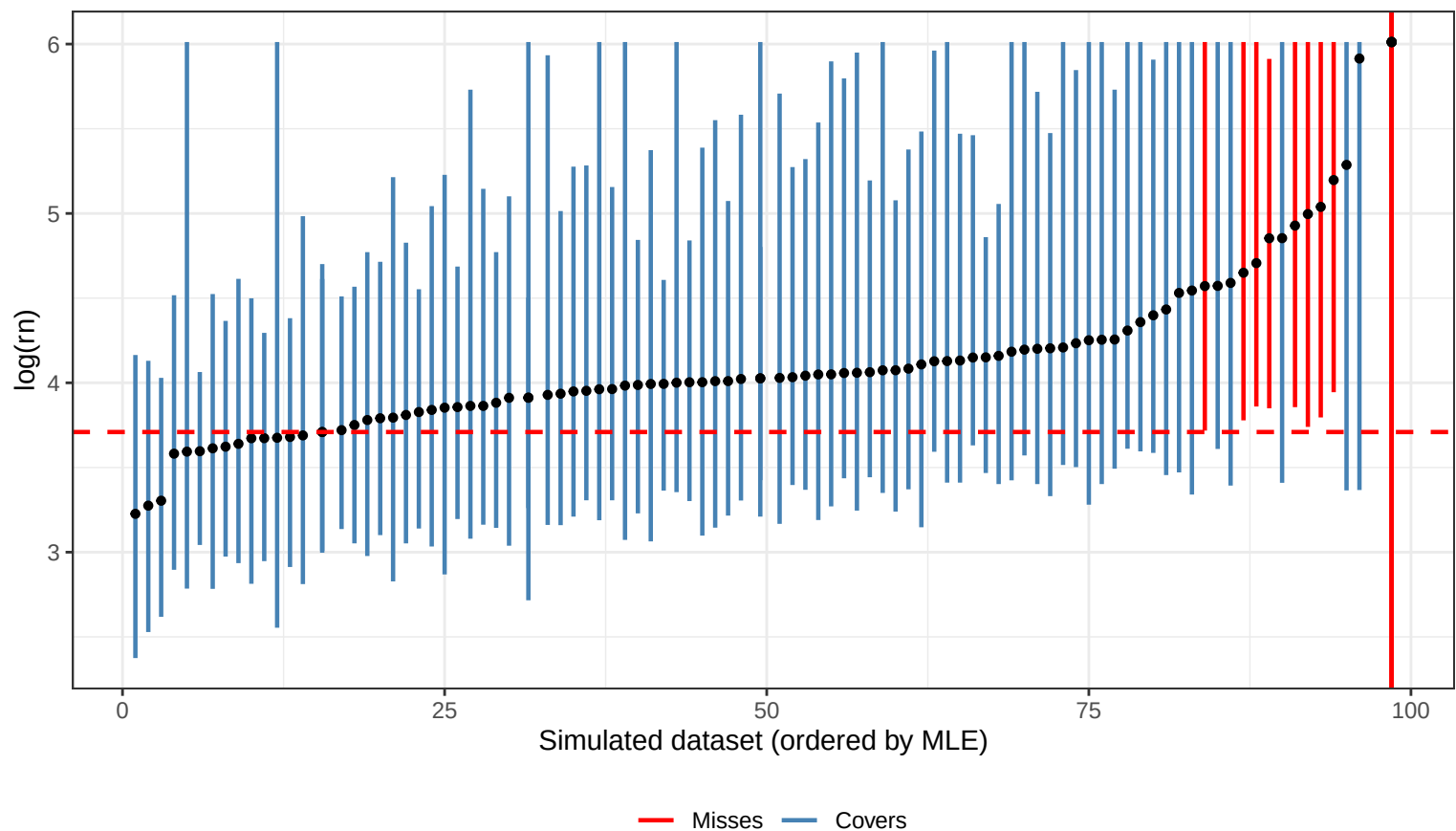
MCAP 95% CI Coverage for rn (88/100 = 88.0%)
