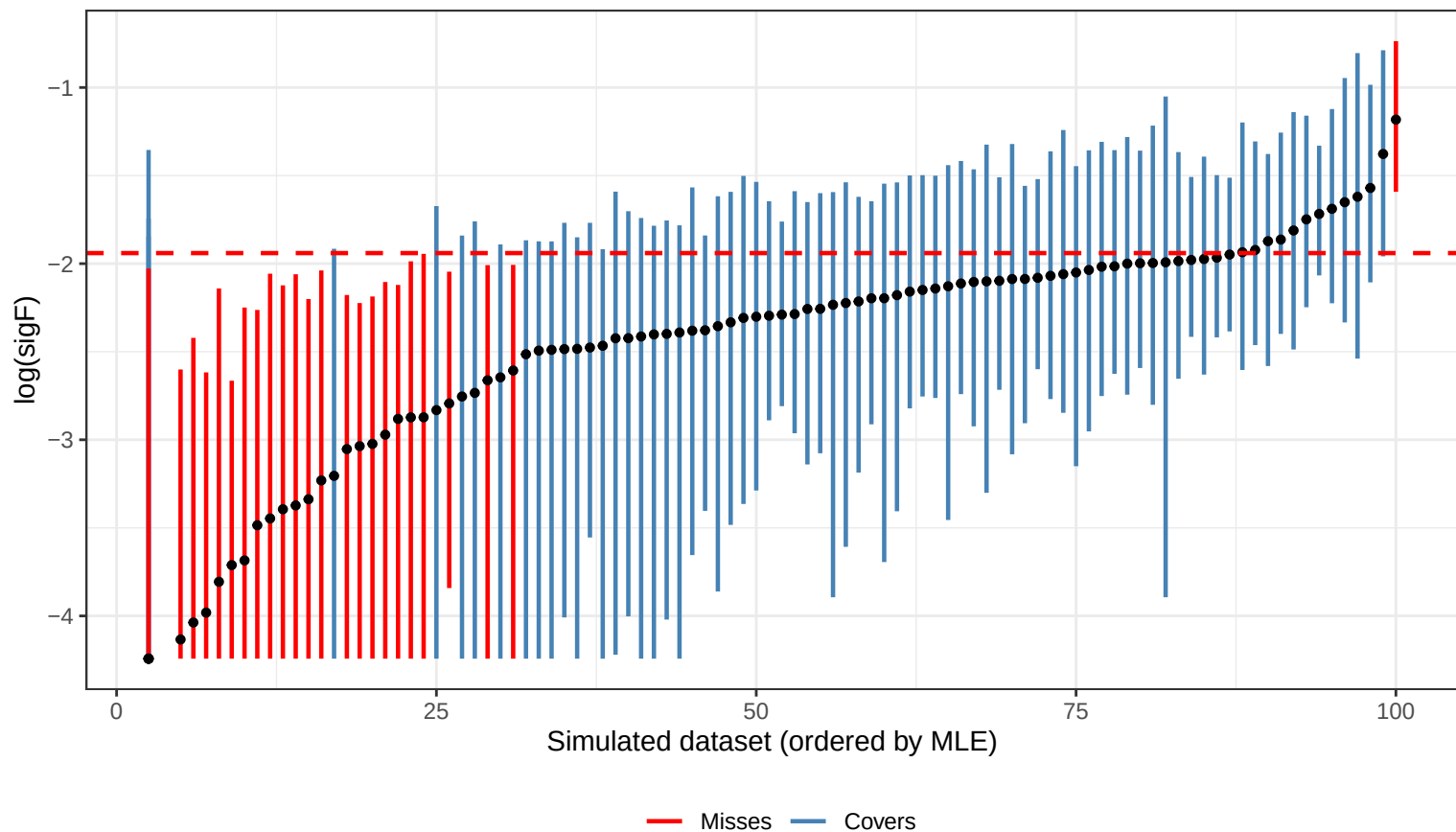
MCAP 95% CI Coverage for sigF (76/100 = 76.0%)
