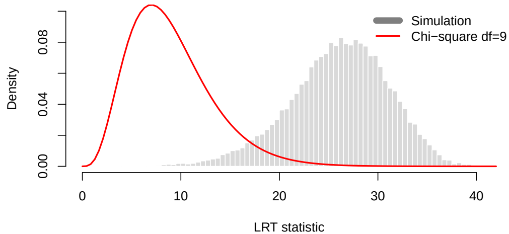
Figure S-2: Histogram of the likelihood ratio statistic (twice the difference of the maximized log-likelihoods) for simulations from H_0 with U = 10 , N = 20 , \sigma = 1 , \tau = 0.5 . The red line shows the chi-square approximation based on Wilks' Theorem.
