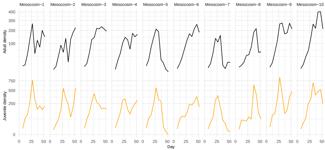
Figure S-21: Density (Individuals/Liter) of D. dentifera . The top panel shows adult susceptibles ( D. dentifera , black). The bottom panel shows juvenile susceptibles ( D. dentifera , orange). There were negligible infected juveniles. Columns are buckets corresponding to replications with same treatment setting.
