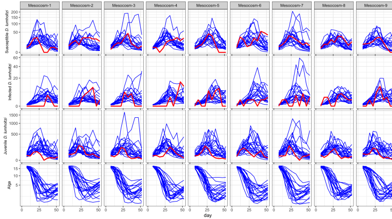
Figure S-14: Simulated trajectories of susceptible D. lumholtzi , infected D. lumholtzi , juvenile D. lumholtzi and alga density ( 10^6 \cdot \text{cells/Liter} ) over time (days) for each experimental unit (u1 to u9). The blue lines represent individual simulation runs, capturing the variability in susceptible density across replicates, while the red line represents the actual experimental data.
