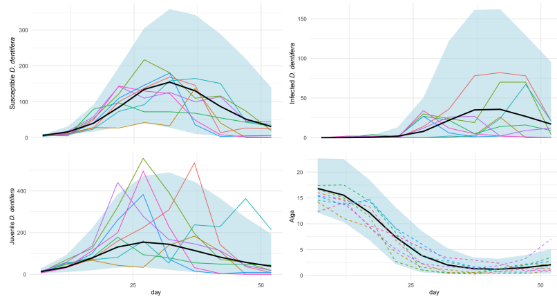
Figure S-11: Simulation plots of densities (Individuals/Liter) for susceptible, infected, and juvenile D. dentifera , along with alga density ( 10^6 ·cells/Liter) and parasite density ( 10^3 ·spores/Liter), over time (days). The colorful solid lines represent observed experimental data, showing the variability across different experimental replicates. The black line represents the mean trajectory from the simulation model, capturing the general trend of each density. The light blue shaded area corresponds to the 95% confidence interval of the simulations, indicating the range of model predictions. Dashed lines illustrate individual simulated trajectories, highlighting the model's ability to capture fluctuations around the mean trajectory.
