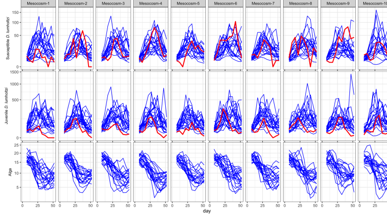
Figure S-28: Simulated densities (Individuals/Liter) of susceptible D. lumholtzi and juvenile D. lumholtzi , with alga density ( 10^6 \cdot \text{cells/Liter} ), for each experimental unit. The blue lines represent individual simulation runs, capturing the variability in susceptible density across replicates, while the red line represents the actual experiment data.
