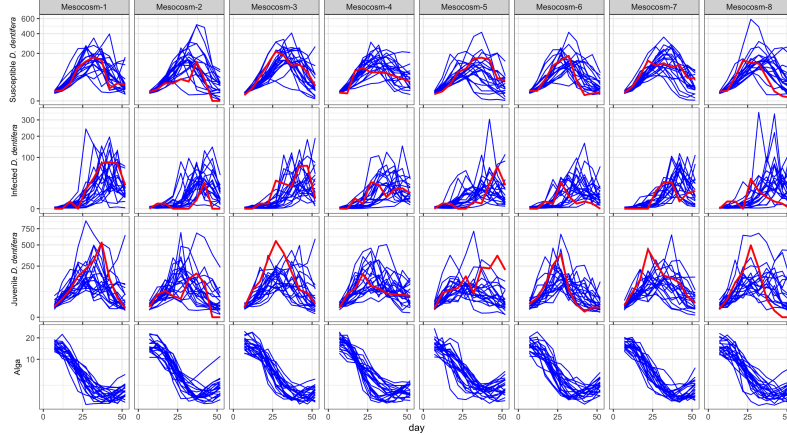
Figure S-12: Simulated densities (Individuals/Liter) of susceptible D. dentifera , infected D. dentifera density, juvenile D. dentifera and alga density ( 10^6 ·cells/Liter) over time (days) for each experimental unit. The blue lines represent individual simulation runs, capturing the variability in susceptible density across replicates, while the red line represents the actual experimental data.
