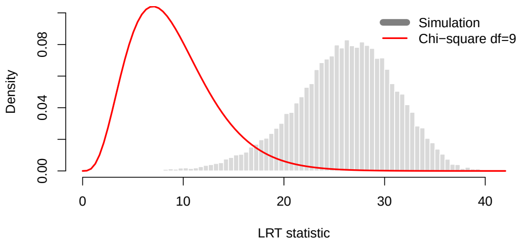
Figure S-2: Histogram of the likelihood ratio statistic (twice the difference of the maximized log-likelihoods) for simulations from H_0 with U = 10 , N = 20 , \sigma = 1 , \tau = 0.5 . The red line shows the chi-square approximation based on Wilks' Theorem.
