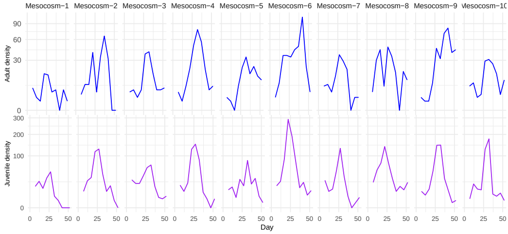
Figure S-22: Density (Individuals/Liter) of D. lumholtzi . The top panel shows adult susceptibles ( D. lumholtzi , blue). The bottom panel shows juvenile susceptibles ( D. lumholtzi , purple). There were negligible infected juveniles. Columns are buckets corresponding to replications with same treatment setting.
