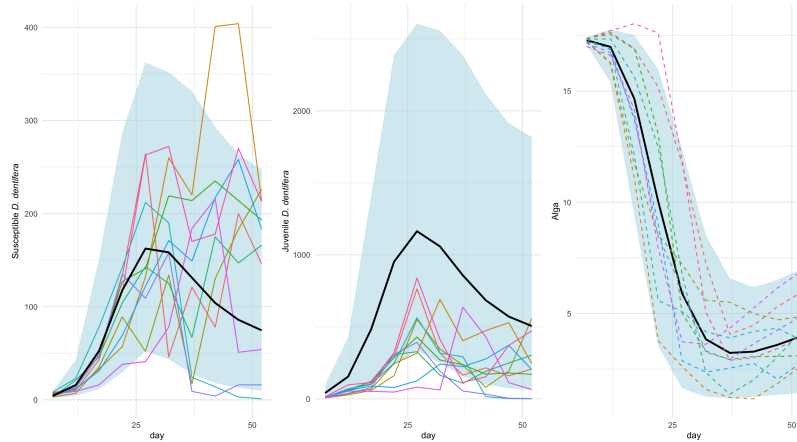
Figure S-25: Simulation plots of densities (Individuals/Liter) for susceptible, and juvenile D. dentifera , along with alga density ( 10^6 cells/Liter) and parasite density ( 10^3 spores/Liter), over time (days). The colorful solid lines represent observed experimental data, showing the variability across different experimental replicates. The black line represents the mean trajectory from the simulation model, capturing the general trend of each density. The light blue shaded area corresponds to the 95% confidence interval of the simulations, indicating the range of model predictions. Dashed lines illustrate individual simulated trajectories, highlighting the model's ability to capture fluctuations around the mean trajectory.
