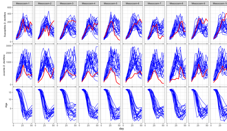
Figure S-26: Simulated densities (Individuals/Liter) of susceptible D. dentifera , juvenile D. dentifera and alga density ( 10^6 cells/Liter) over time (days) for each experimental unit. The blue lines represent individual simulation runs, capturing the variability in susceptible density across replicates, while the red line represents the actual experiment data.
