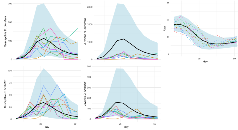
Figure S-18: Simulation plots of densities (Individuals/Liter) for susceptible and juvenile populations of both native D. dentifera and invasive D. lumholtzi , along with alga density ( 10^6 cells/Liter) over time (days). Colorful solid lines represent observed experimental data for each experimental replicate, showcasing variability across replicates. The black line represents the mean simulation trajectory, while the light blue shaded area corresponds to the 95% confidence interval of the simulation. Dashed lines indicate individual simulation cases, illustrating the model's capacity to capture fluctuations around the mean trajectory.
