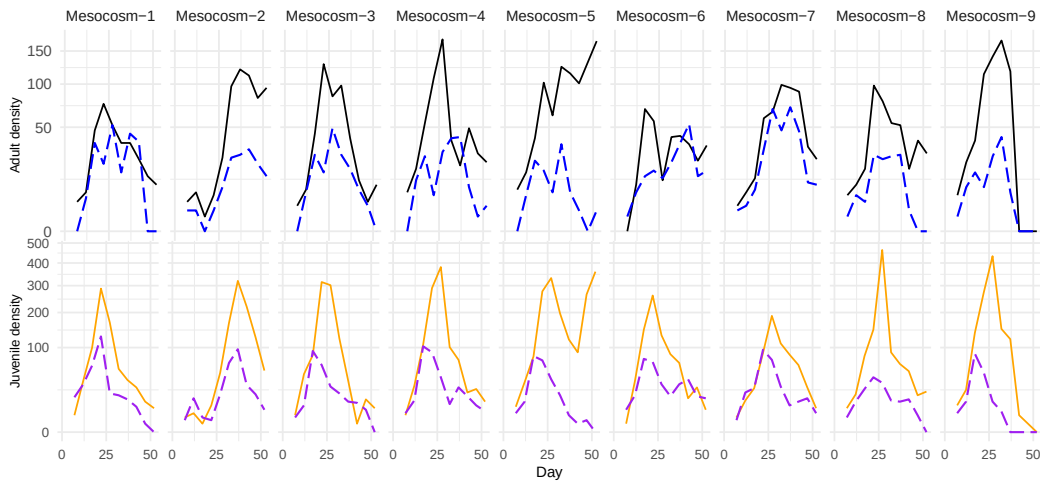
Figure S-16: Density (Individuals/Liter) of D. dentifera (solid lines) and D. lumholtzi (dashed lines). The top panel shows adult susceptibles ( D. dentifera , black and D. lumholtzi , blue). The bottom panel shows juvenile susceptibles ( D. dentifera , orange; D. lumholtzi , purple). There were negligible infected juveniles. Columns are buckets corresponding to replications with same treatment setting.
