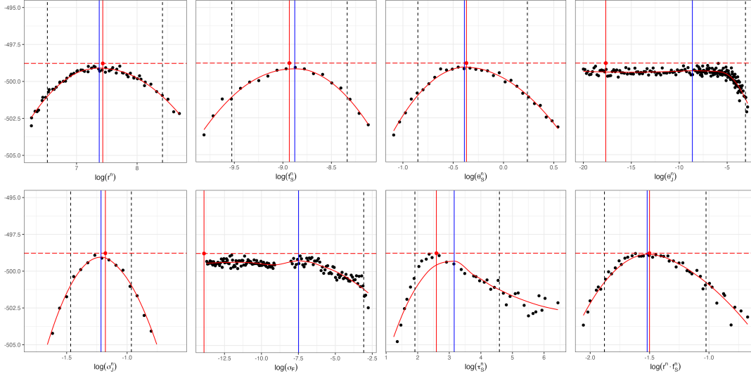
Figure S-23: Monte Carlo Adjusted Profile results of SRJF model for D. dentifera -only dynamics. The vertical dotted lines represent the 95% confidence interval obtained by MCAP. The vertical blue lines show the MLE estimated using MCAP. The red vertical lines correspond to the model with the overall highest likelihood among all searches.
