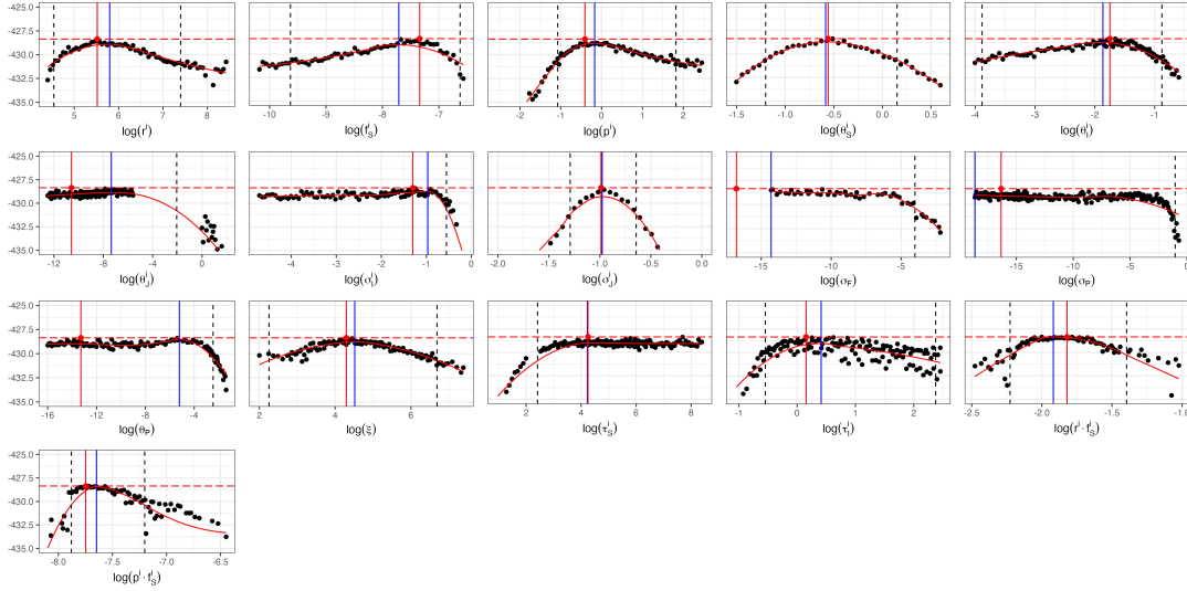
Figure S-10: Monte Carlo Adjusted Profile results of SIRJPF model for D. lumholtzi -only dynamics. The vertical dotted lines represent the 95% confidence interval obtained by MCAP. The vertical blue lines show the MLE estimated using MCAP. The red vertical lines correspond to the model with the overall highest likelihood among all searches.
