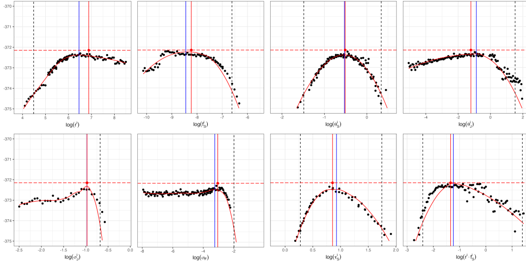
Figure S-24: Monte Carlo Adjusted Profile results of SRJF model for D. lumholtzi -only dynamics. The vertical dotted lines represent the 95% confidence interval obtained by MCAP. The vertical blue lines show the MLE estimated using MCAP. The red vertical lines correspond to the model with the overall highest likelihood among all searches.
