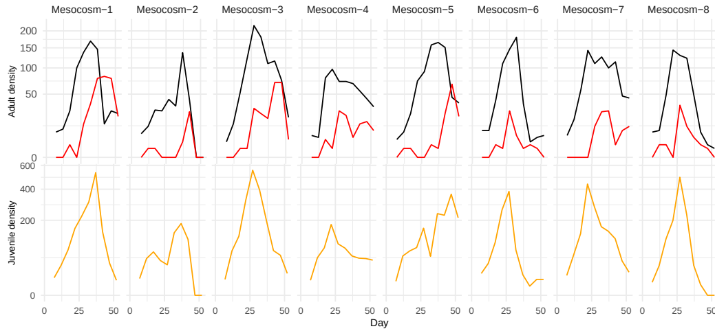
Figure S-7: Density (Individuals/Liter) of D. dentifera . The top panel shows adult susceptibles ( D. dentifera , black) and infecteds ( D. dentifera , red). The bottom panel shows juvenile susceptibles ( D. dentifera , orange). There were negligible infected juveniles. Columns are buckets corresponding to replications with same treatment setting.
