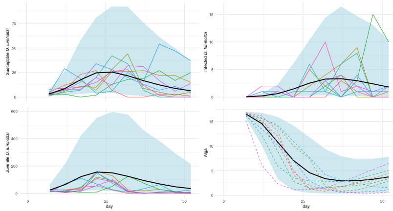
Figure S-13: Simulation plots of densities (Individuals/Liter) for susceptible, infected, and juvenile D. lumholtzi , along with alga density ( 10^6 \cdot \text{cells/Liter} ) and parasite density ( 10^3 \cdot \text{spores/Liter} ), over time (days). The colorful solid lines represent observed experimental data, showing the variability across different experimental replicates. The black line represents the mean trajectory from the simulation model, capturing the general trend of each density. The light blue shaded area corresponds to the 95% confidence interval of the simulations, indicating the range of model predictions. Dashed lines illustrate individual simulated trajectories, highlighting the model's ability to capture fluctuations around the mean trajectory.
