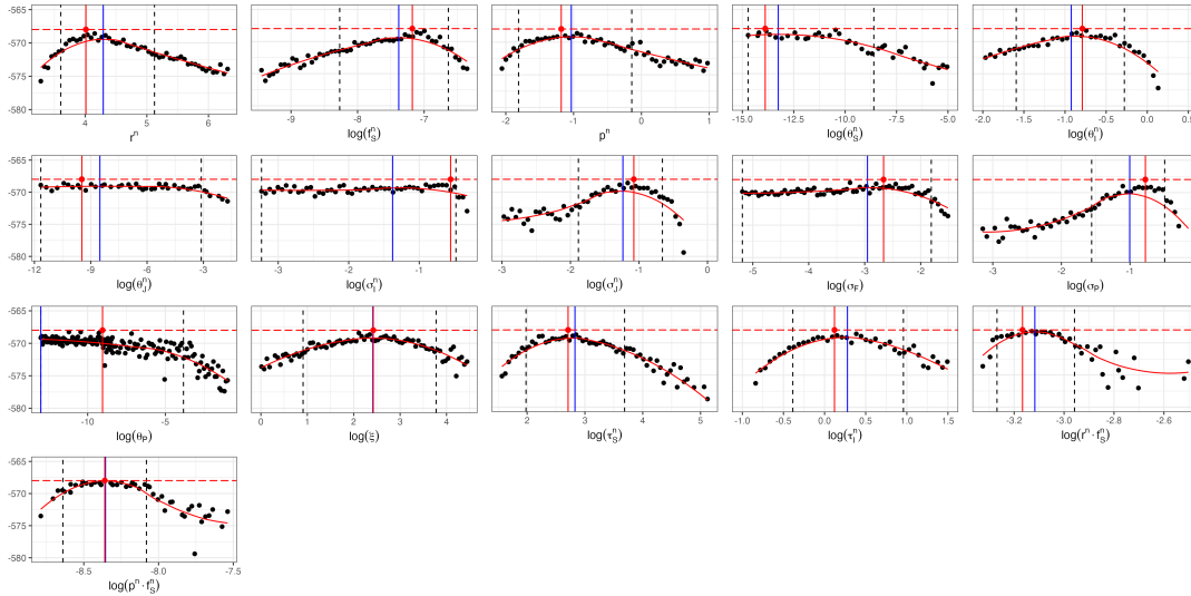
Figure S-9: Monte Carlo Adjusted Profile results of SIRJPF model for D. dentifera -only dynamics. The vertical dotted lines represent the 95% confidence interval obtained by MCAP. The vertical blue lines show the MLE estimated using MCAP. The red vertical lines correspond to the model with the overall highest likelihood among all searches.
