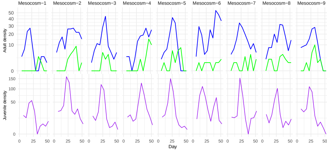
Figure S-8: Density (Individuals/Liter) of D. lumholtzi . The top panel shows adult susceptibles ( D. lumholtzi , blue) and infecteds ( D. lumholtzi , green). The bottom panel shows juvenile susceptibles ( D. lumholtzi , purple). There were negligible infected juveniles. Columns are buckets corresponding to replications with same treatment setting.
