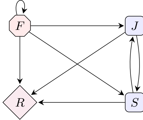
Figure S-20: Flow diagram for the SRJF model illustrating population interactions. The model includes the R state, representing mortality. For \mathbb{k} \in \{\mathfrak{m}, \mathfrak{i}\} , susceptible populations ( S^{\mathbb{k}} ) can reproduce into juvenile ( J^{\mathbb{k}} ) and A. Algae ( F ) will be refilled, as shown by the recycling arrows. Both S^{\mathbb{k}} and J^{\mathbb{k}} consume resources from F , and over time, components in F also progress to R .
