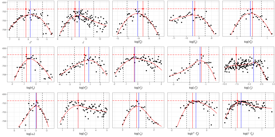
Figure S-17: Monte Carlo Adjusted Profile results of SRJF2 model for dynamics with both species of Daphnia . The vertical dotted lines represent the 95% confidence interval obtained by MCAP. The vertical blue lines show the MLE estimated using MCAP. The red vertical lines correspond to the model with the overall highest likelihood among all searches.
