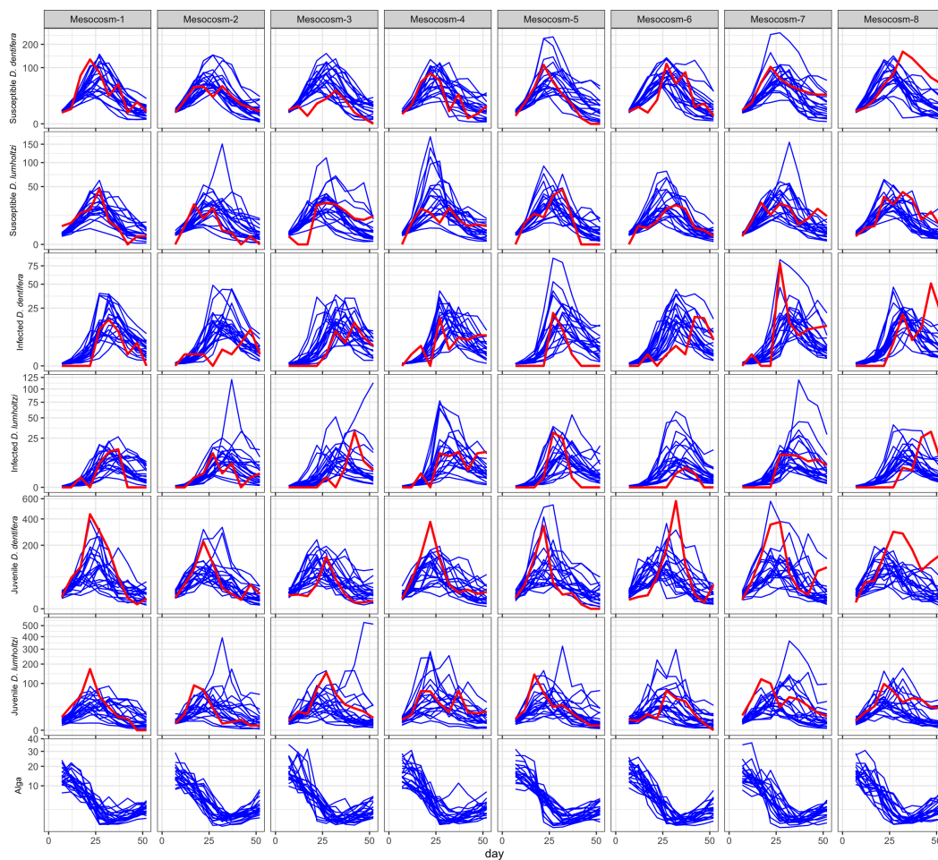
Figure S-3: Simulated densities (Individuals/Liter) of susceptible, infected and juvenile D. dentifera , susceptible, infected and juvenile D. lumholtzi and alga density ( 10^6 ·cells/Liter) over time for each experimental unit. The blue lines represent individual simulation runs, capturing the variability in susceptible density across replicates, while the red line represents the actual experiment data.
