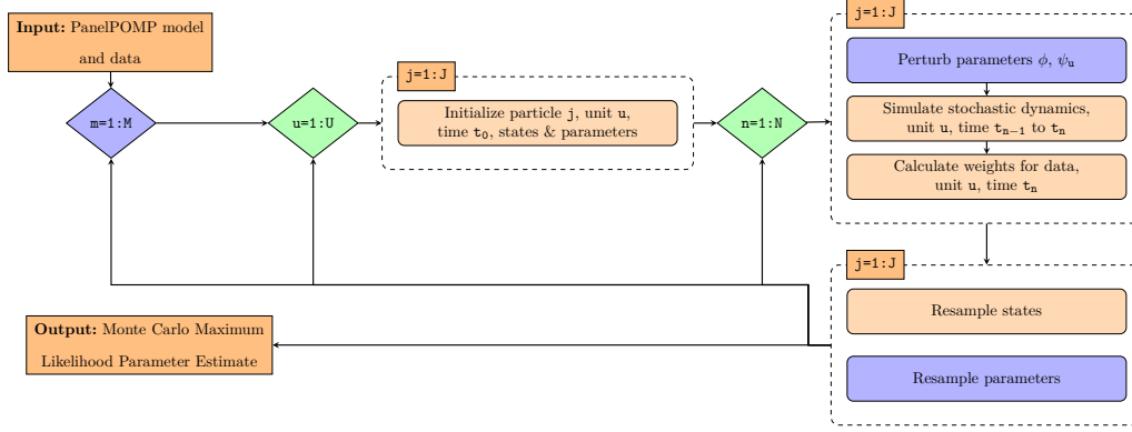
Figure 3: A flow diagram for panel iterated filtering. If the blue shaded blocks are omitted, this becomes a standard particle filter for each unit. Full pseudocode is in Section S2. In the PIF algorithm of Bretó et al. (2020), the parameter resampling step involves re-selecting the unit-specific parameters corresponding to particle j for units \tilde{u} \neq u as well as \psi_u . For the marginalized PIF algorithm, only \phi and \psi_u are reselected in this step.
