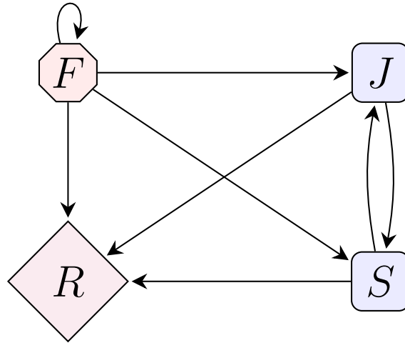
Figure S-18: Flow diagram for the SRJF model illustrating population interactions. The model includes the R state, representing mortality. For k \in \{\mathfrak{m}, \mathfrak{i}\} , susceptible populations ( S^k ) can reproduce into juvenile ( J^k ) and A. Algae ( F ) will be refilled, as shown by the recycling arrows. Both S^k and J^k consume resources from F , and over time, components in F also progress to R .
