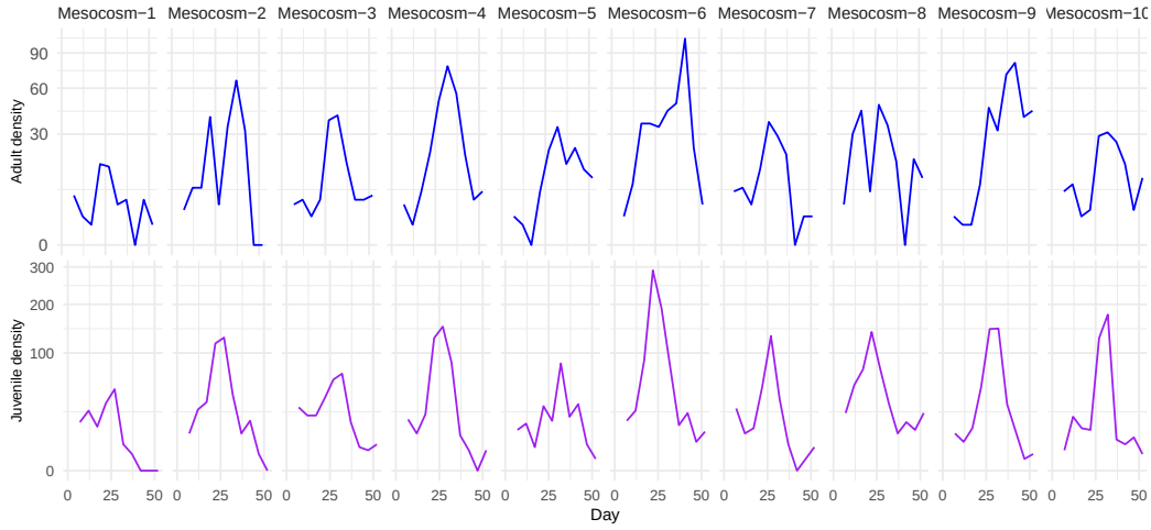
Figure S-21: Density (Individuals/Liter) of D. lumholtzi . The top panel shows adult susceptibles ( D. lumholtzi , blue). The bottom panel shows juvenile susceptibles ( D. lumholtzi , purple). There were negligible infected juveniles. Columns are buckets corresponding to replications with same treatment setting.
