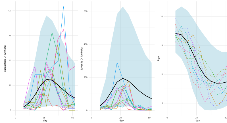
Figure S27: Simulation plots of densities (Individuals/Liter) for susceptible, and juvenile D. lumholtzi , along with alga density ( 10^6 cells/Liter) and parasite density ( 10^3 spores/Liter), over time (days). The colorful solid lines represent observed experimental data, showing the variability across different experimental replicates. The black line represents the mean trajectory from the simulation model, capturing the general trend of each density. The light blue shaded area corresponds to the 95% confidence interval of the simulations, indicating the range of model predictions. Dashed lines illustrate individual simulated trajectories, highlighting the model's ability to capture fluctuations around the mean trajectory.
