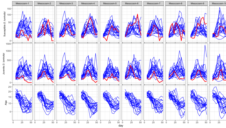
Figure S28: Simulated densities (Individuals/Liter) of susceptible D. lumholtzi and juvenile D. lumholtzi , with alga density ( 10^6 \cdot \text{cells/Liter} ), for each experimental unit. The blue lines represent individual simulation runs, capturing the variability in susceptible density across replicates, while the red line represents the actual experiment data.
