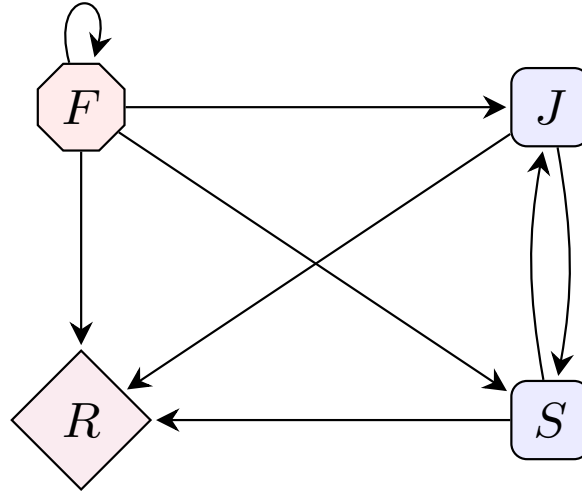
Figure S20: Flow diagram for the SRJF model illustrating population interactions. The model includes the R state, representing mortality. For k \in \{m, i\} , susceptible populations ( S^k ) can reproduce into juvenile ( J^k ) and A. Algae ( F ) will be refilled, as shown by the recycling arrows. Both S^k and J^k consume resources from F , and over time, components in F also progress to R .
