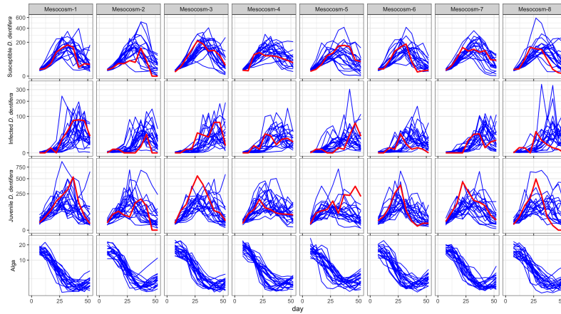
Figure S12: Simulated densities (Individuals/Liter) of susceptible D. dentifera , infected D. dentifera density, juvenile D. dentifera and alga density ( 10^6 ·cells/Liter) over time (days) for each experimental unit. The blue lines represent individual simulation runs, capturing the variability in susceptible density across replicates, while the red line represents the actual experimental data.
