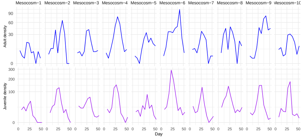
Figure S22: Density (Individuals/Liter) of D. lumholtzi . The top panel shows adult susceptibles ( D. lumholtzi , blue). The bottom panel shows juvenile susceptibles ( D. lumholtzi , purple). There were negligible infected juveniles. Columns are buckets corresponding to replications with same treatment setting.
