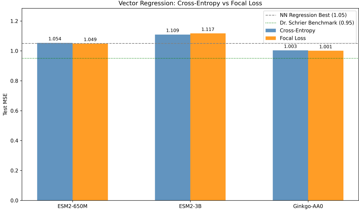
Figure 3: Vector regression results comparing three PLM embedding types and two loss functions. Ensemble MSE values are annotated above each bar.
