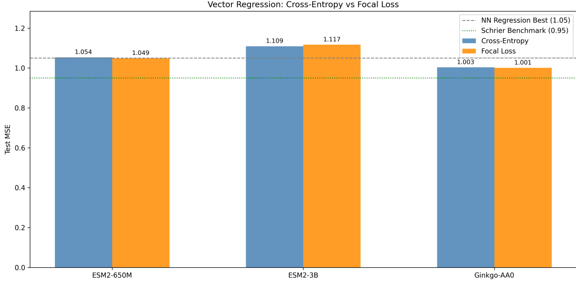
Figure 3: Vector regression results comparing three PLM embedding types and two loss functions. Ensemble MSE values are annotated above each bar.
